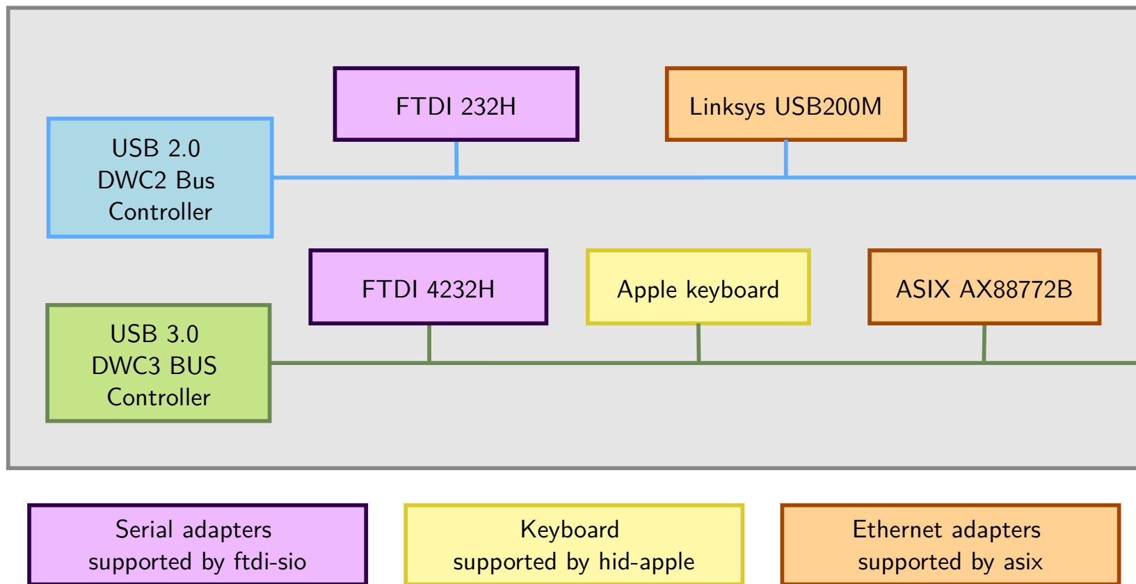
Hardware view of the bus
