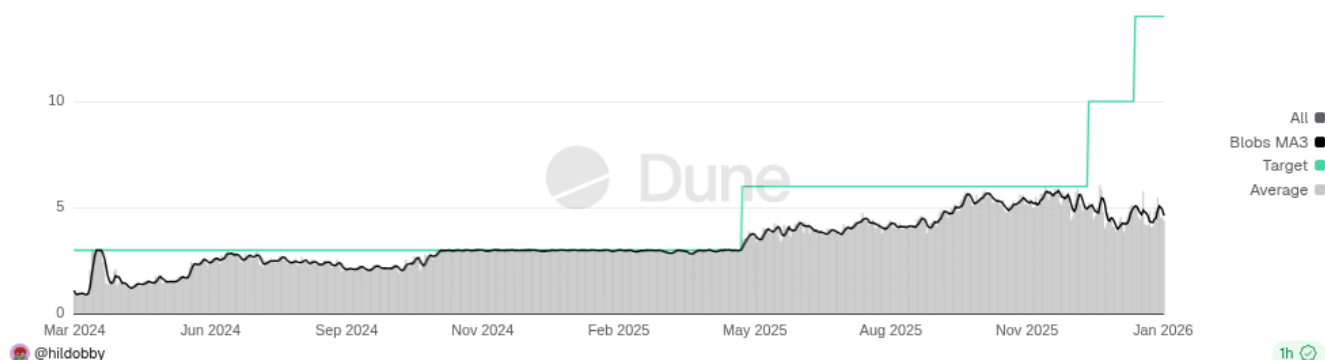
Average Blob Count per Block Since Dencun
