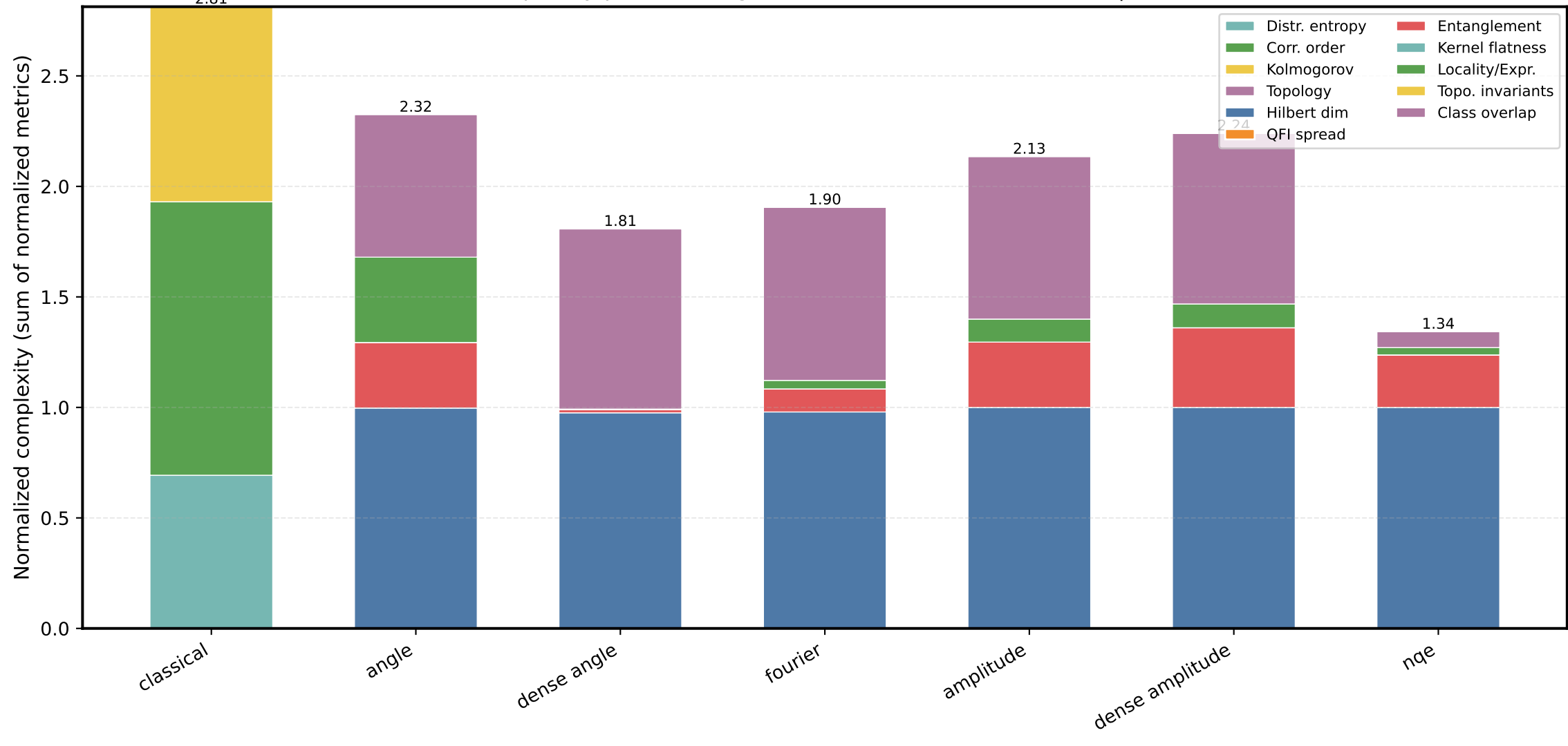
Dataset complexity per encoding (normalized metrics) — fashion | classes: full
