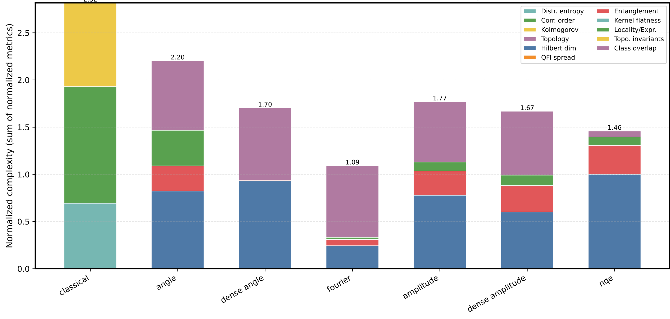
Dataset complexity per encoding (normalized metrics) — kmnist | classes: full
