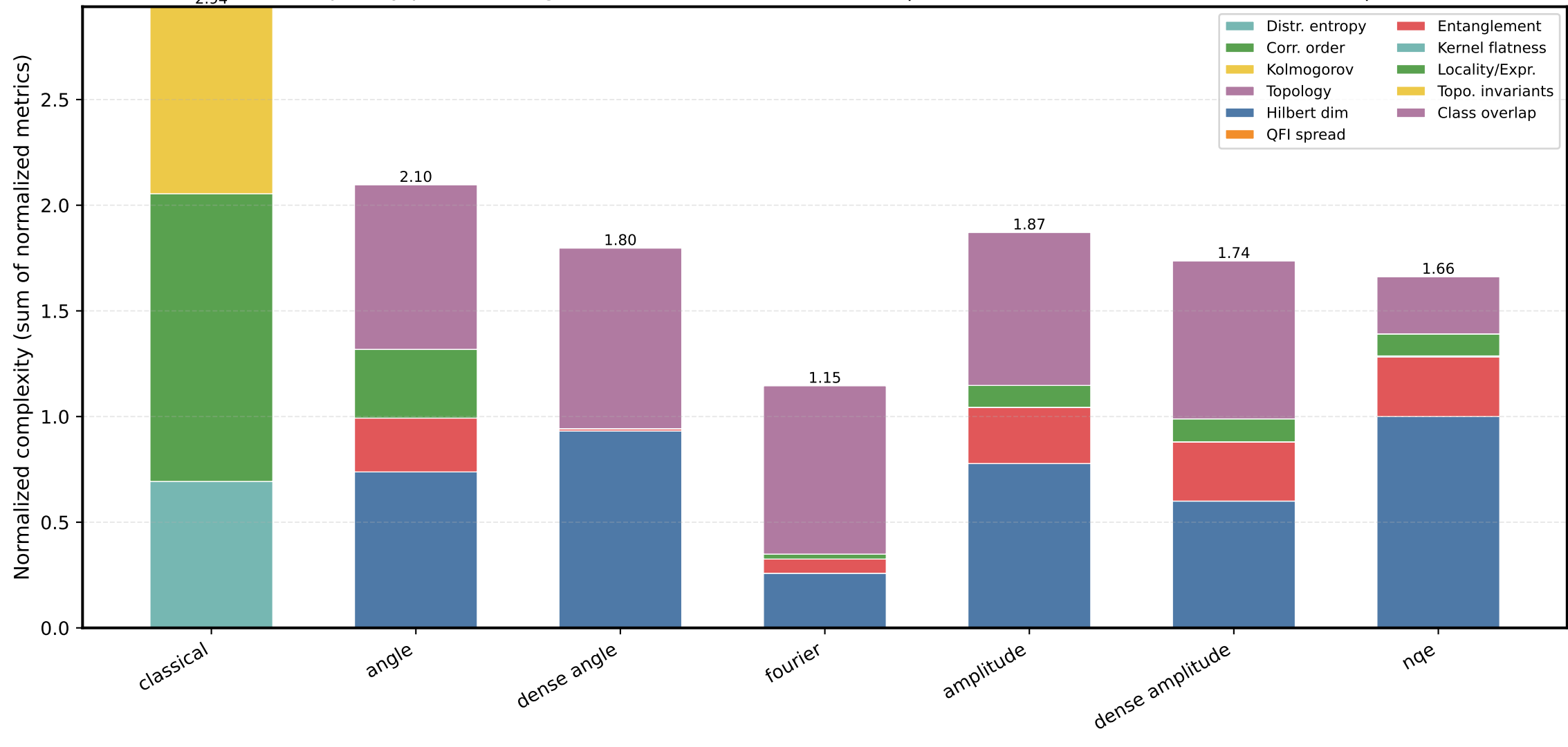
Dataset complexity per encoding (normalized metrics) — mnist | classes: (0, 1, 2, 3, 4, 5, 6, 7, 8, 9, 10) | PCA→8
