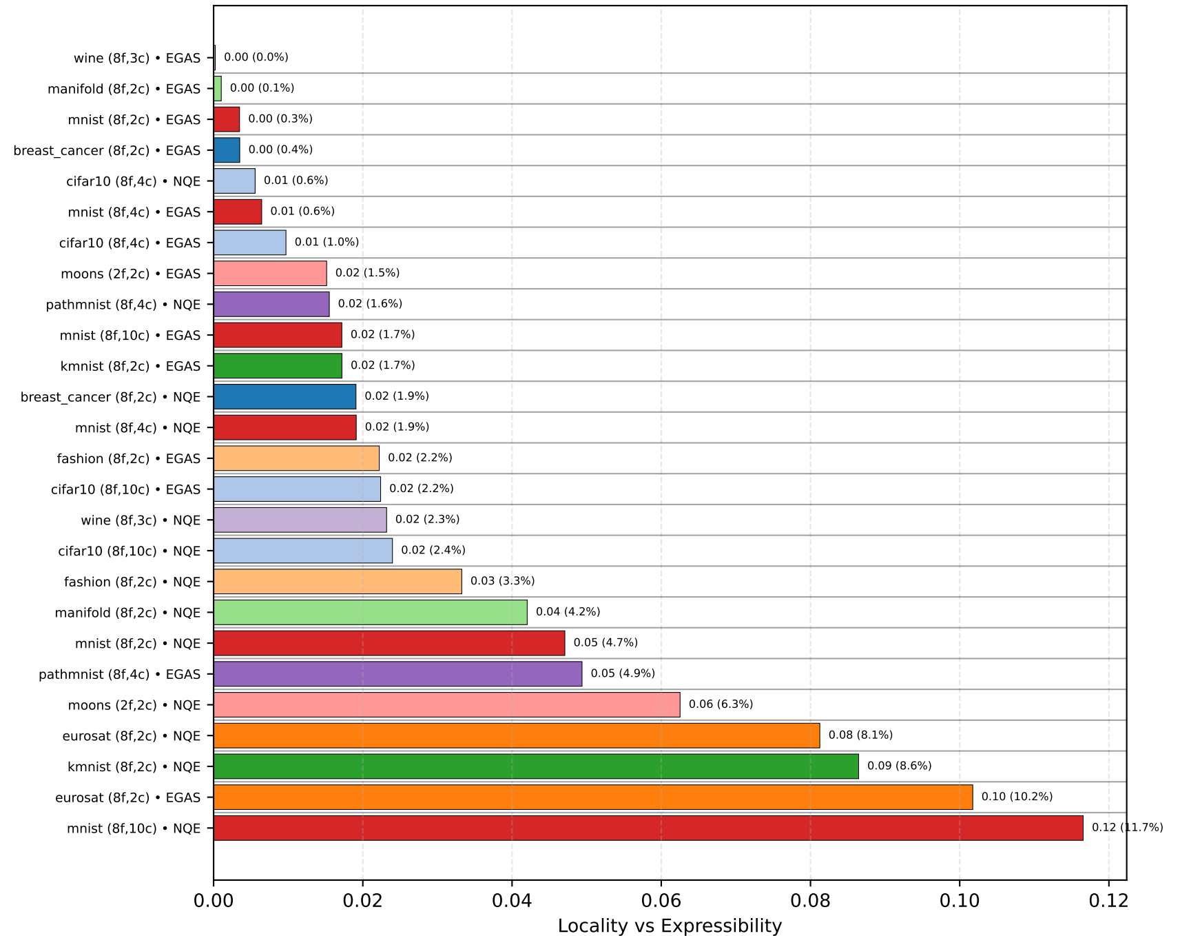
Locality vs Expressibility
