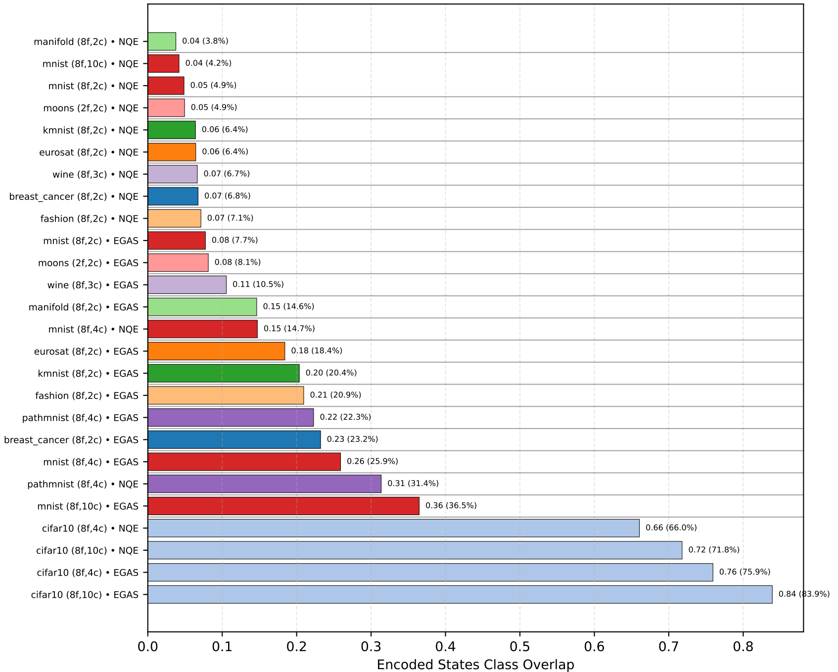
Encoded States Class Overlap
