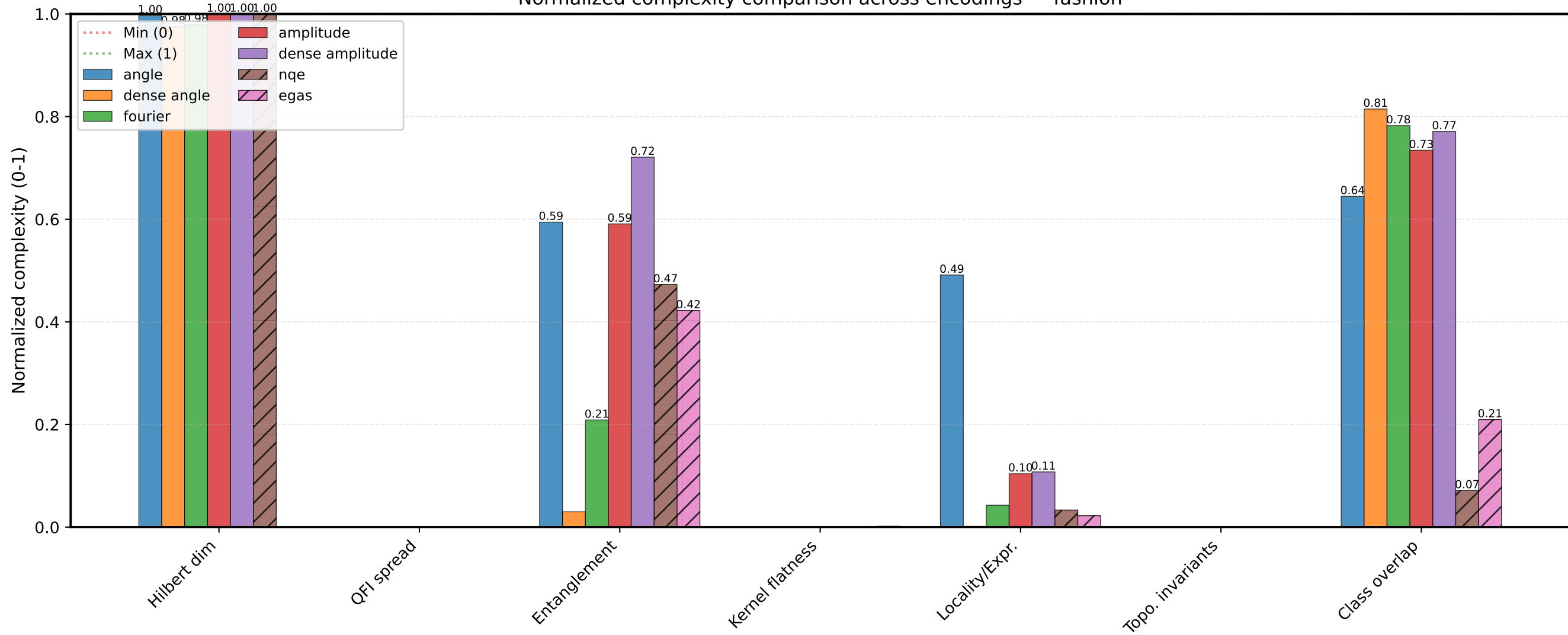
Normalized complexity comparison across encodings — fashion
