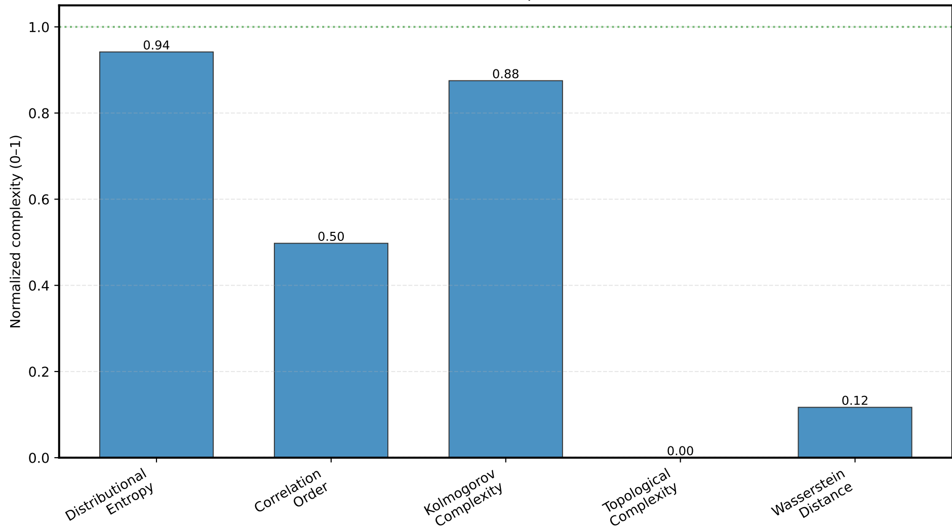
Normalized dataset complexities — eurosat
