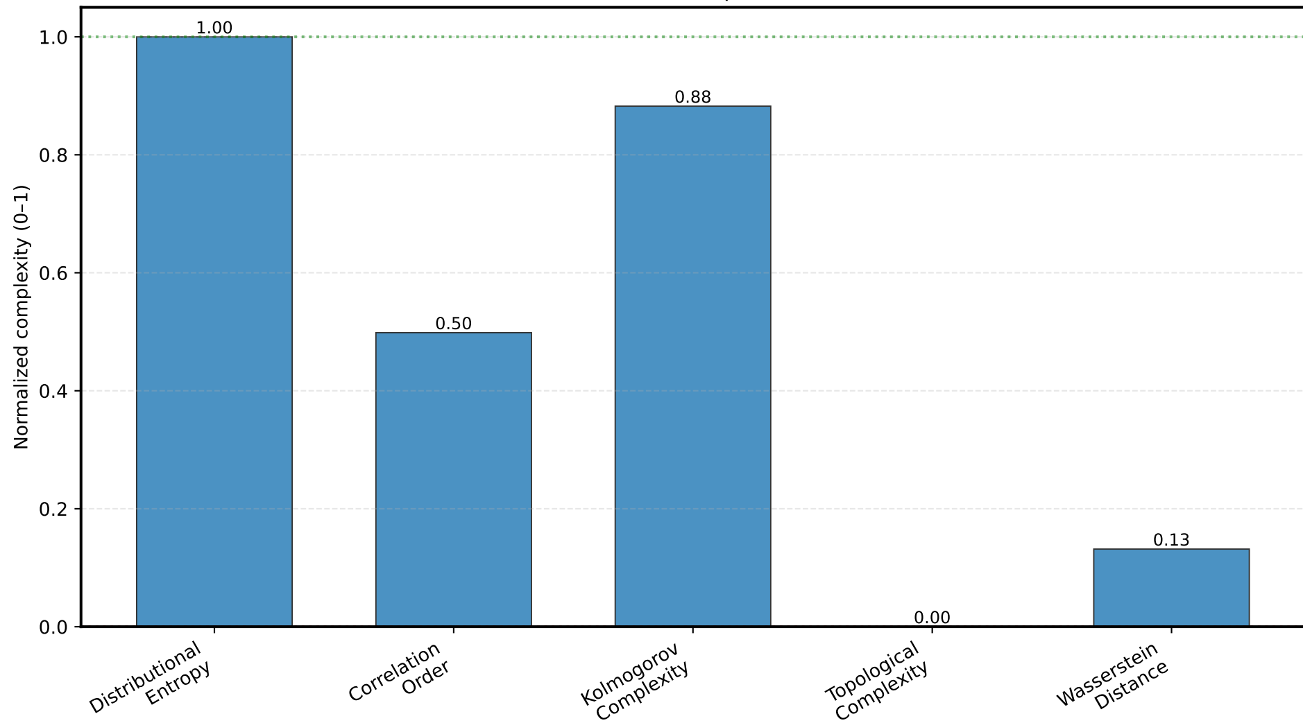
Normalized dataset complexities — fashion
