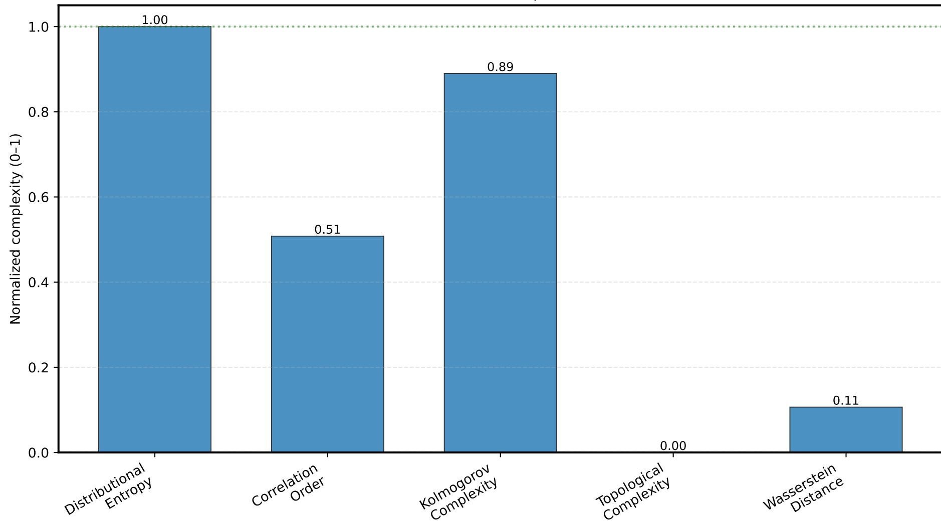
Normalized dataset complexities — wine
