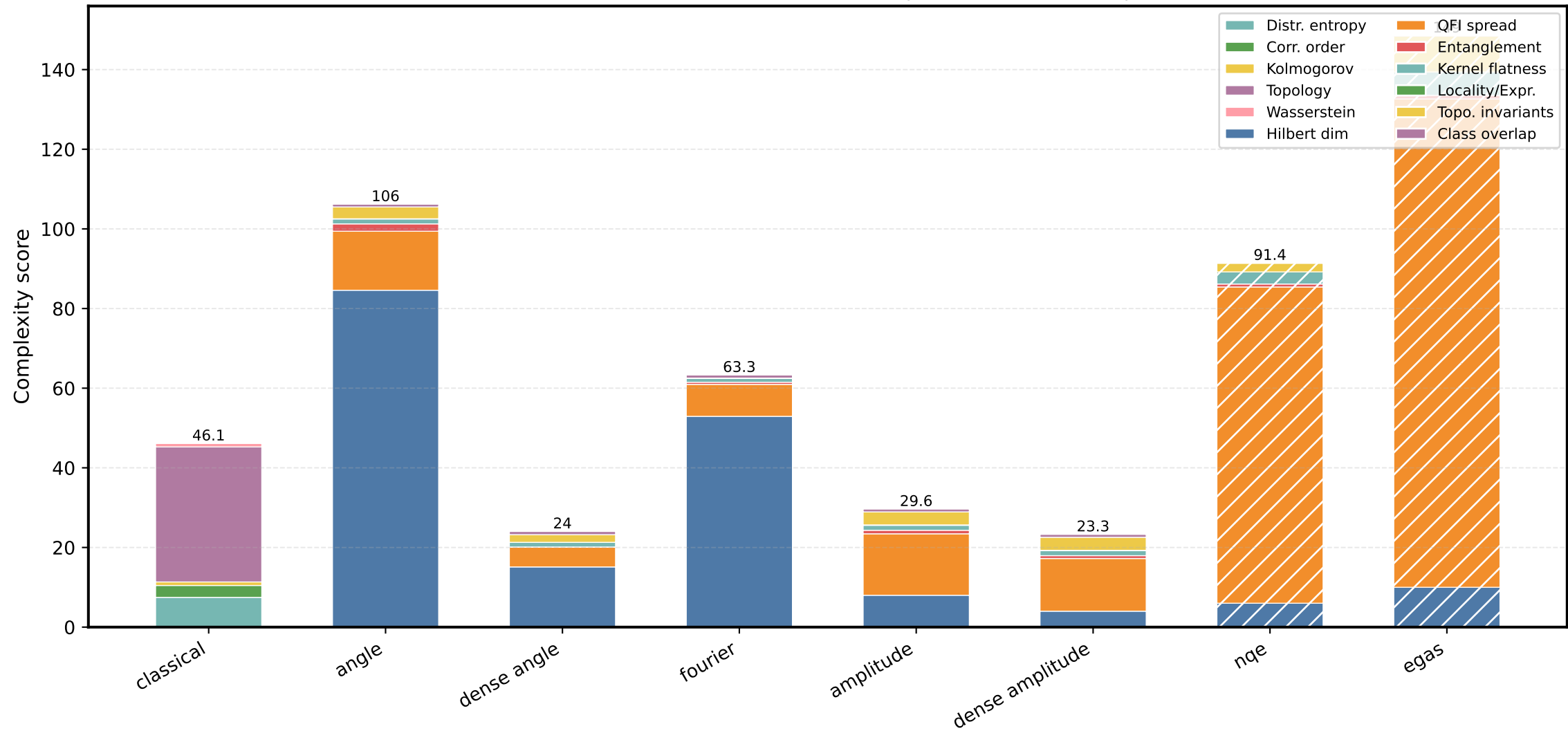
Dataset complexity per encoding — wine | classes: (0, 1, 2) | PCA→8
