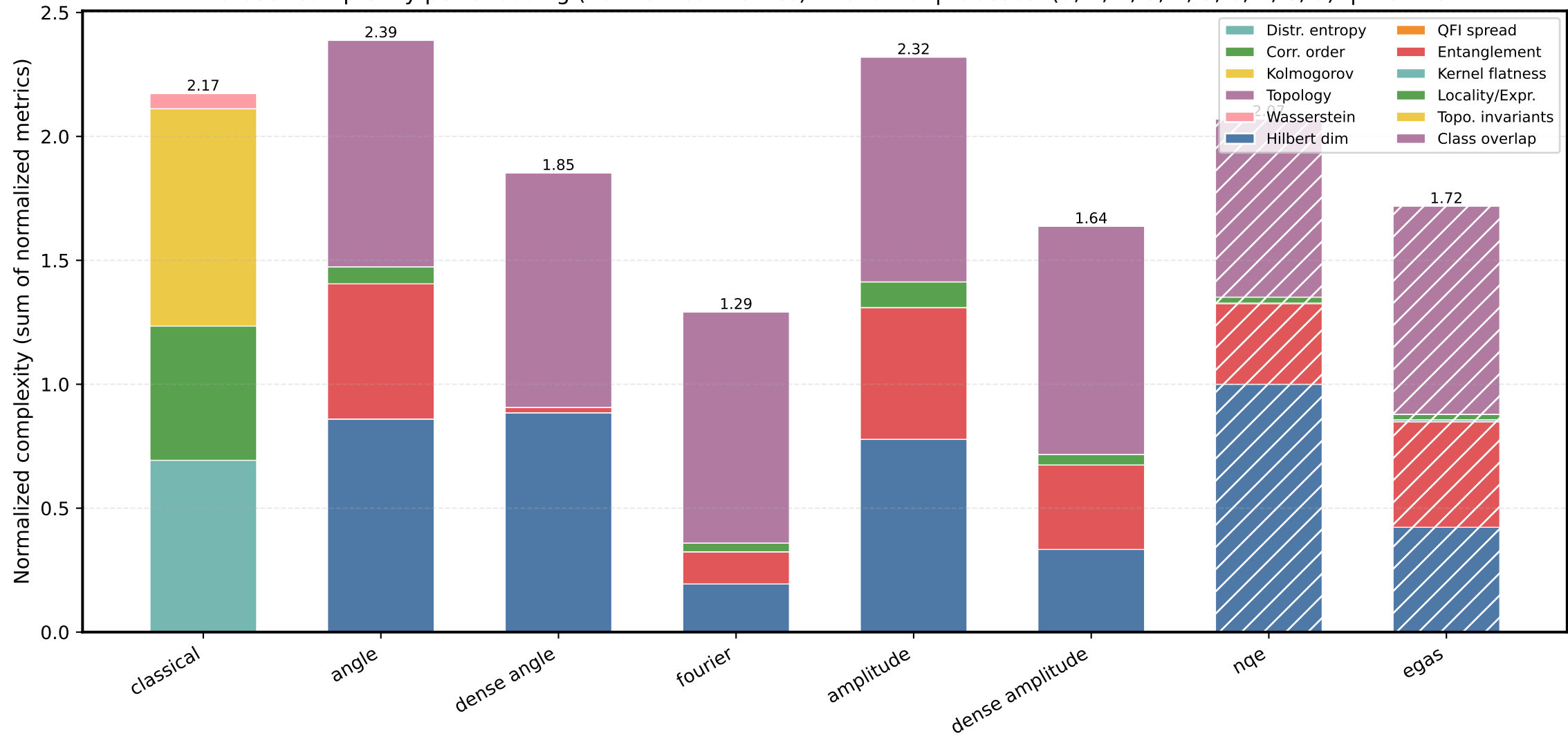
Dataset complexity per encoding (normalized metrics) — cifar10 | classes: (0, 1, 2, 3, 4, 5, 6, 7, 8, 9) | PCA→8
