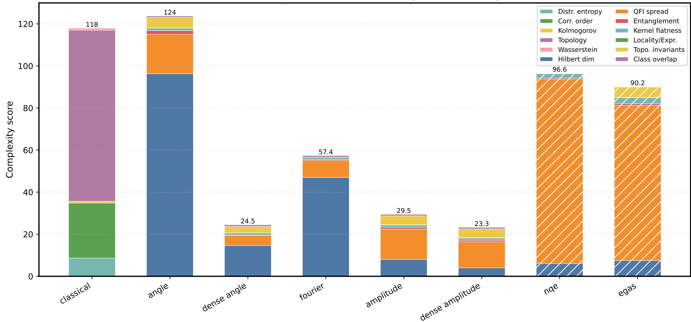
Dataset complexity per encoding — eurosat | classes: (0, 1) | PCA→8
