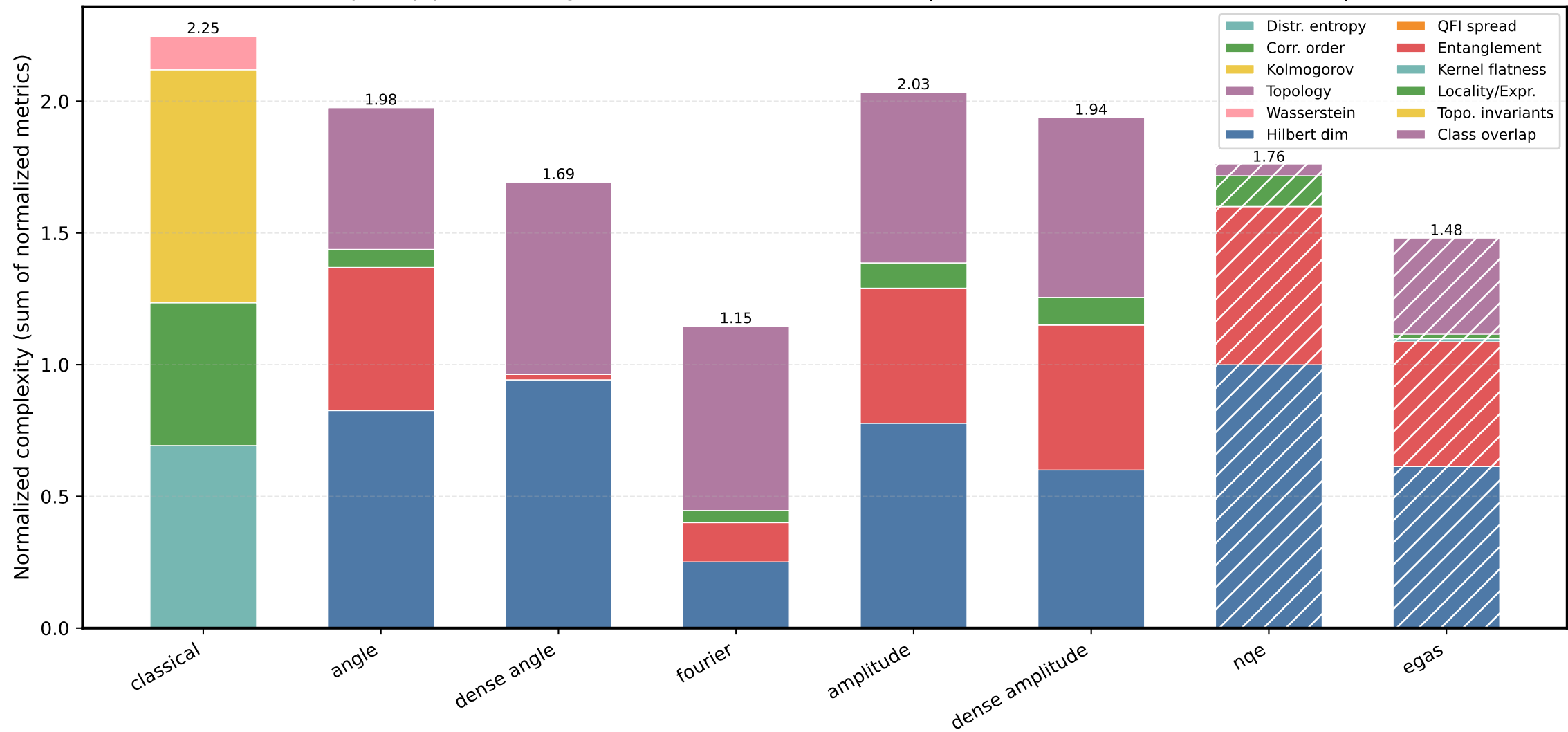
Dataset complexity per encoding (normalized metrics) — mnist | classes: (0, 1, 2, 3, 4, 5, 6, 7, 8, 9) | PCA→8
