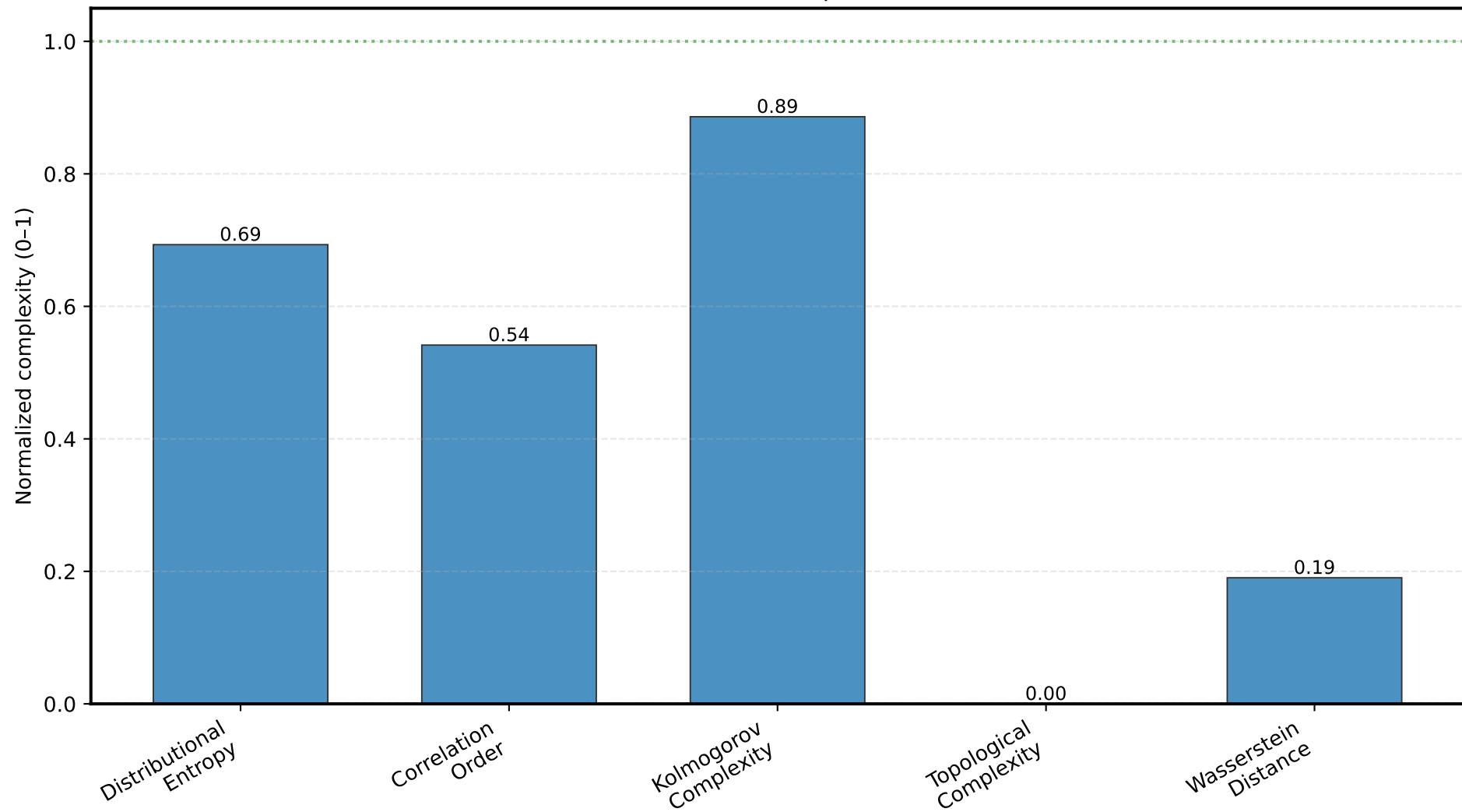
Normalized dataset complexities — mnist
