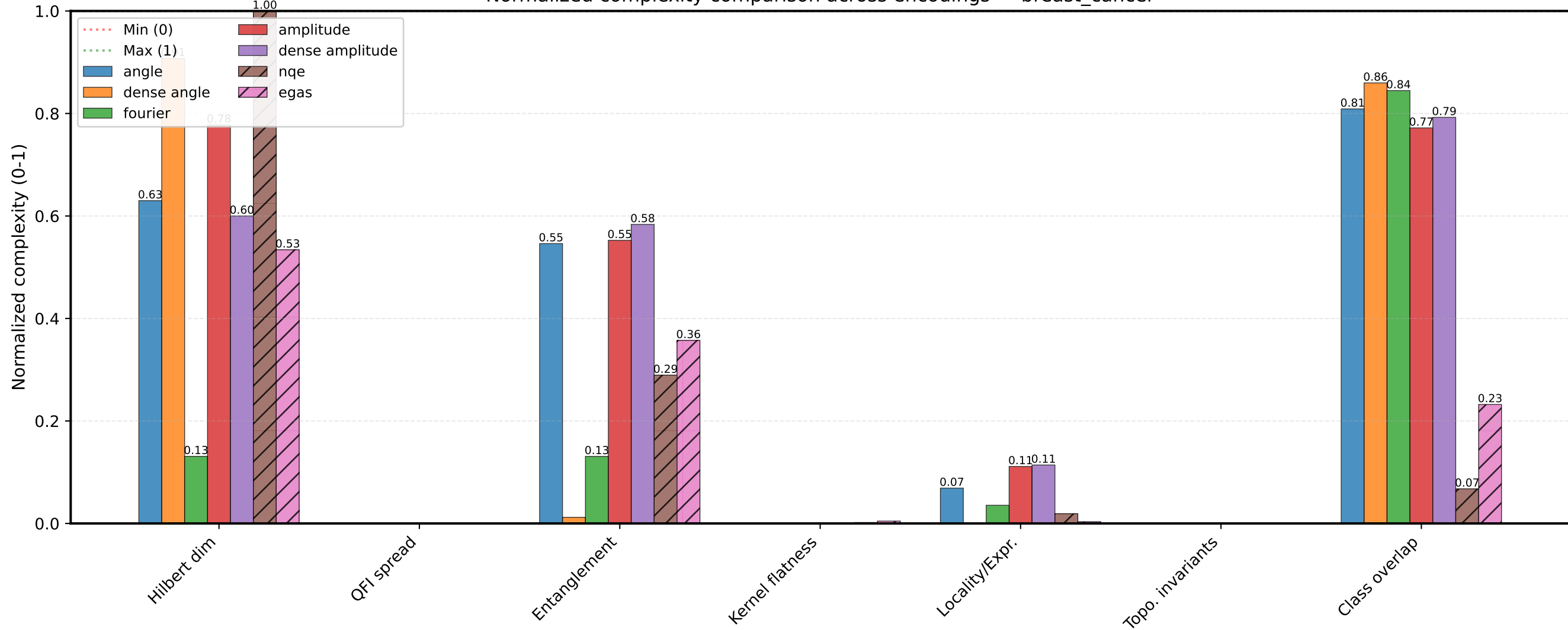
Normalized complexity comparison across encodings — breast_cancer
