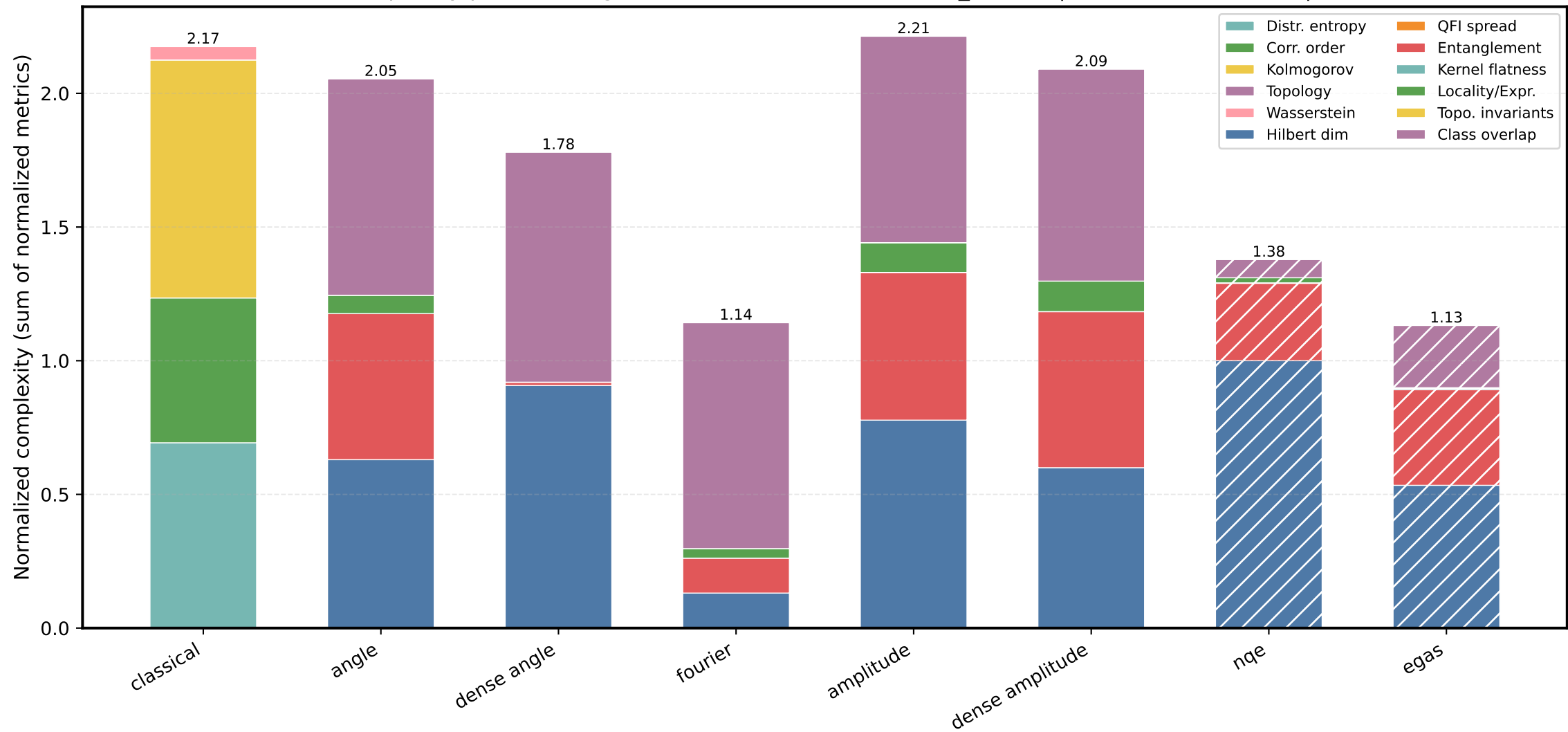
Dataset complexity per encoding (normalized metrics) — breast_cancer | classes: (0, 1, 2, 3) | PCA→8
