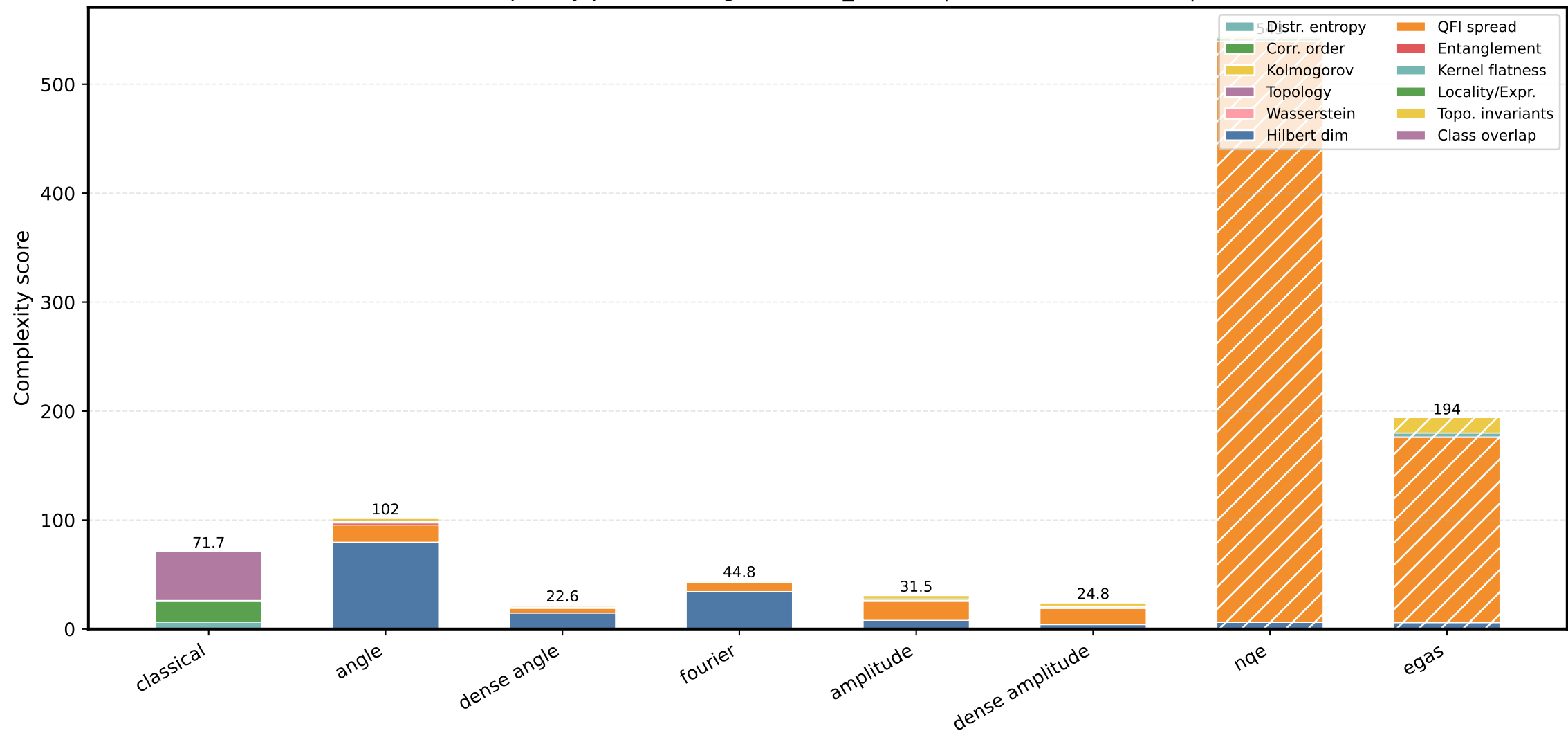
Dataset complexity per encoding — breast_cancer | classes: (0, 1, 2, 3) | PCA→8
