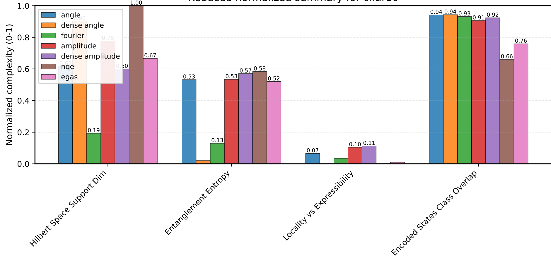
Reduced normalized summary for cifar10
