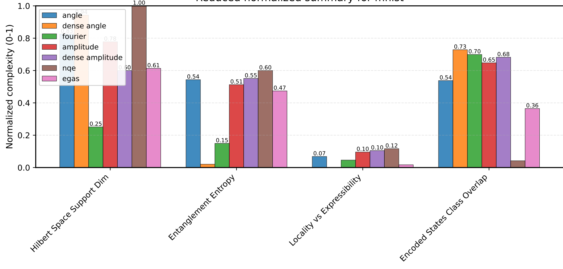
Reduced normalized summary for mnist
