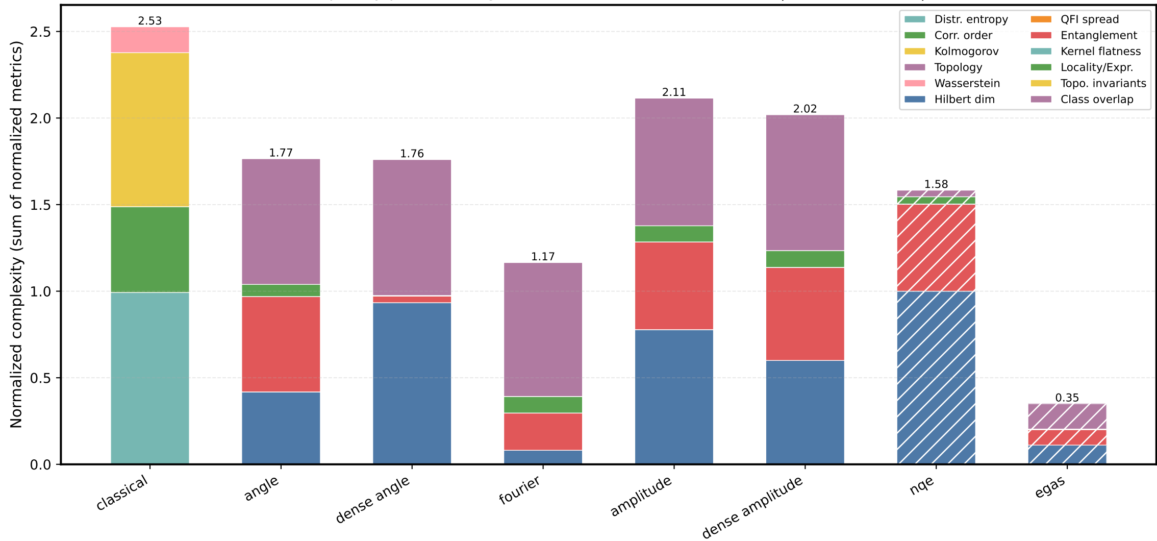
Dataset complexity per encoding (normalized metrics) — manifold | classes: (0, 1) | PCA→8
