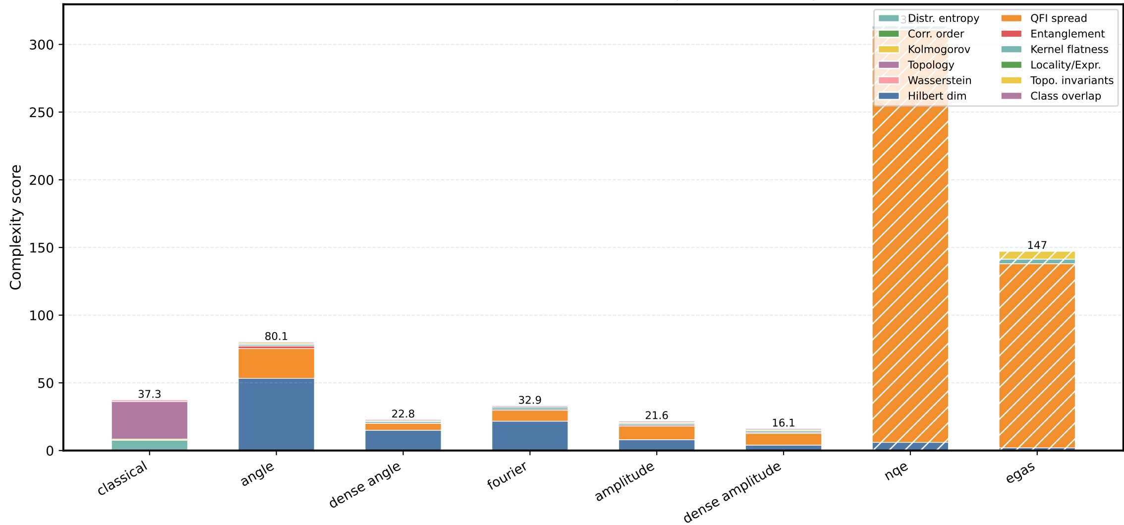
Dataset complexity per encoding — manifold | classes: (0, 1) | PCA→8
