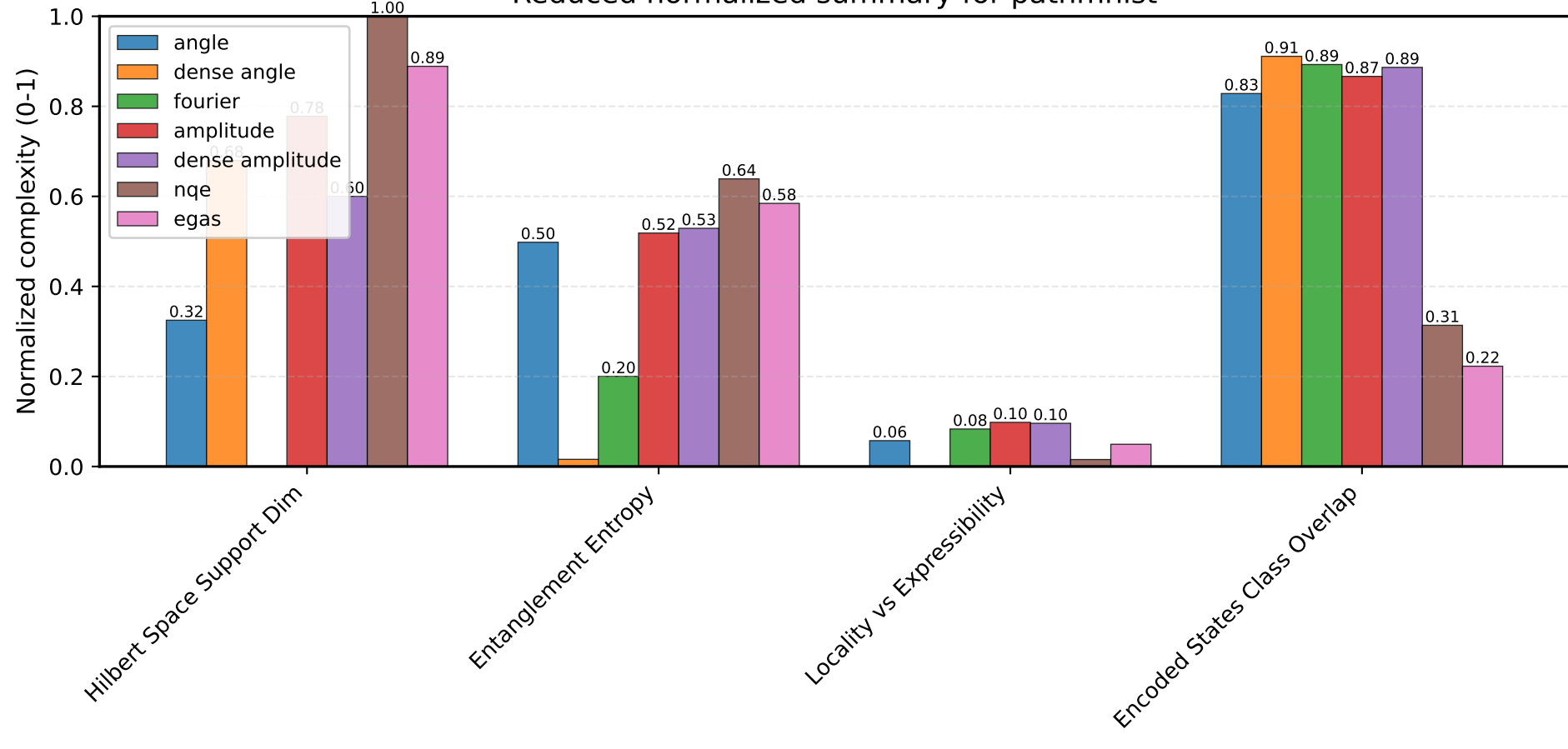
Reduced normalized summary for pathmnist
