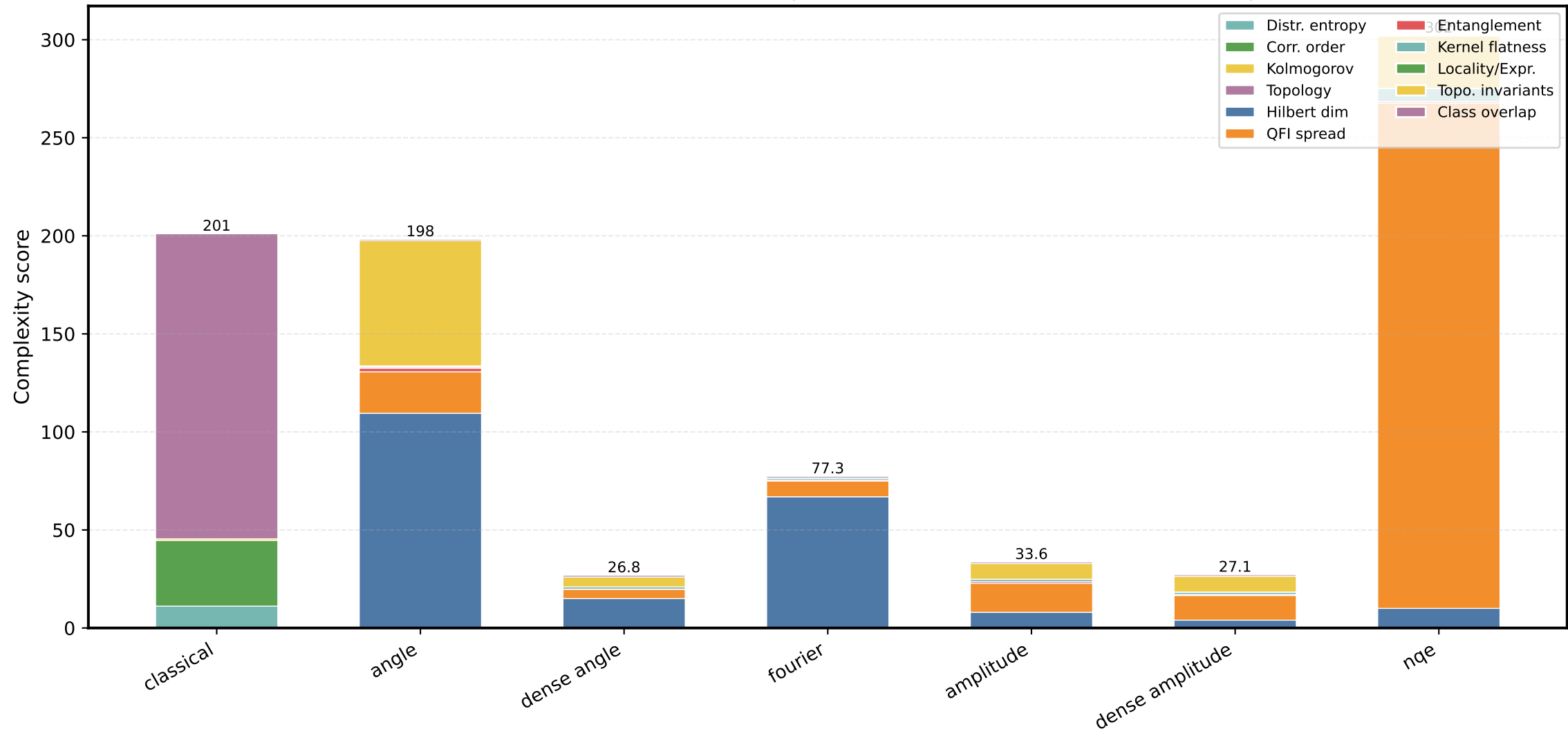
Dataset complexity per encoding — mnist | classes: (0, 1, 2, 3, 4, 5, 6, 7, 8, 9, 10) | PCA→8
