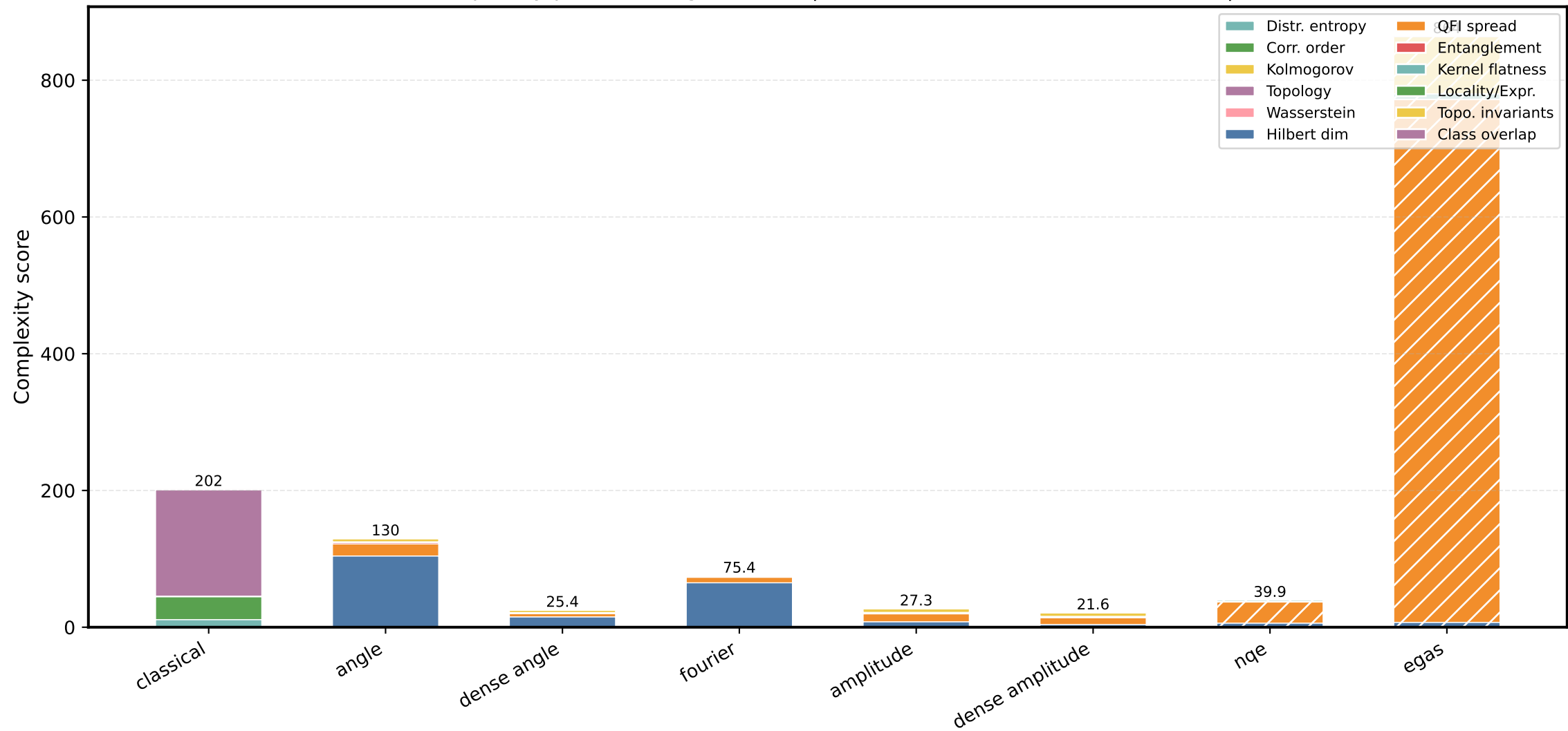
Dataset complexity per encoding — mnist | classes: (0, 1, 2, 3, 4, 5, 6, 7, 8, 9) | PCA→8
