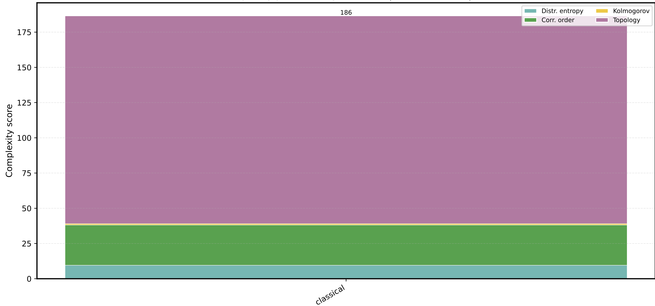
Dataset complexity per encoding — kmnist | classes: (0, 1) | PCA→8
