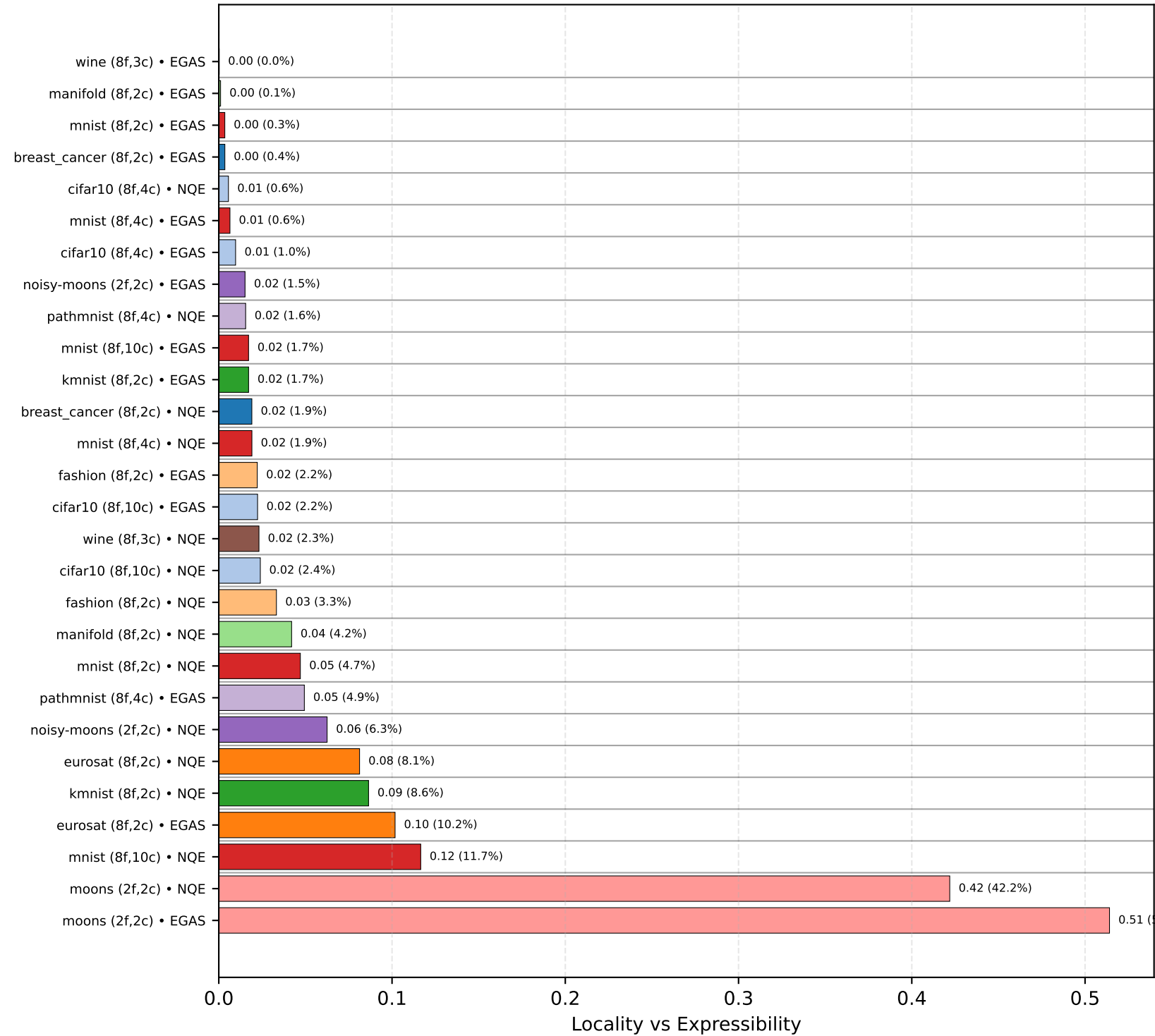
Locality vs Expressibility
