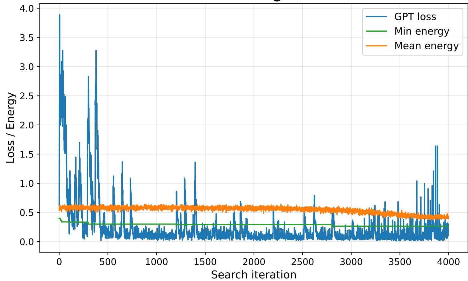
EGAS Training Curve
