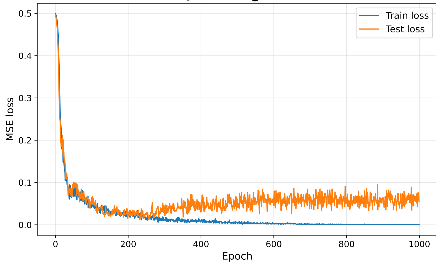
NQE Training Curve
