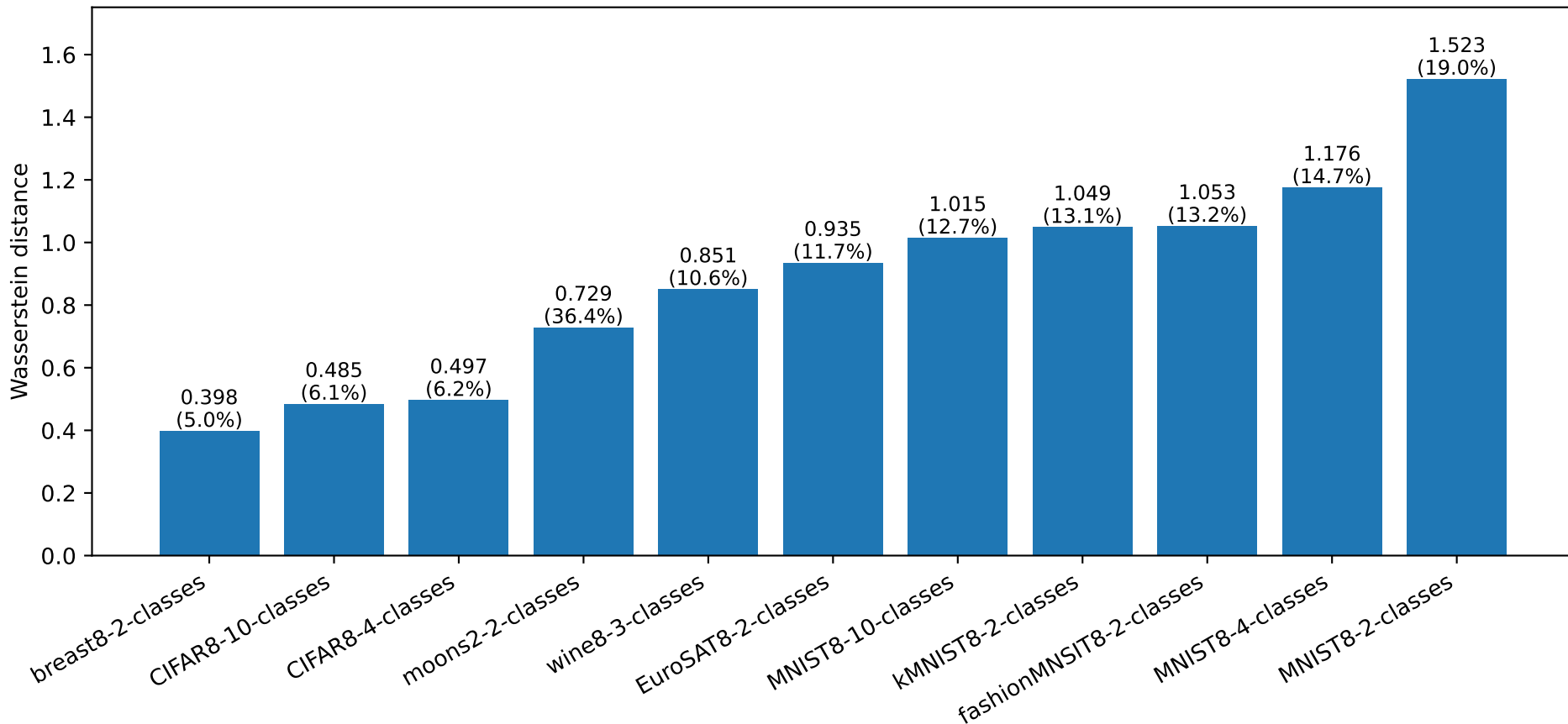
Classical Wasserstein Distance
