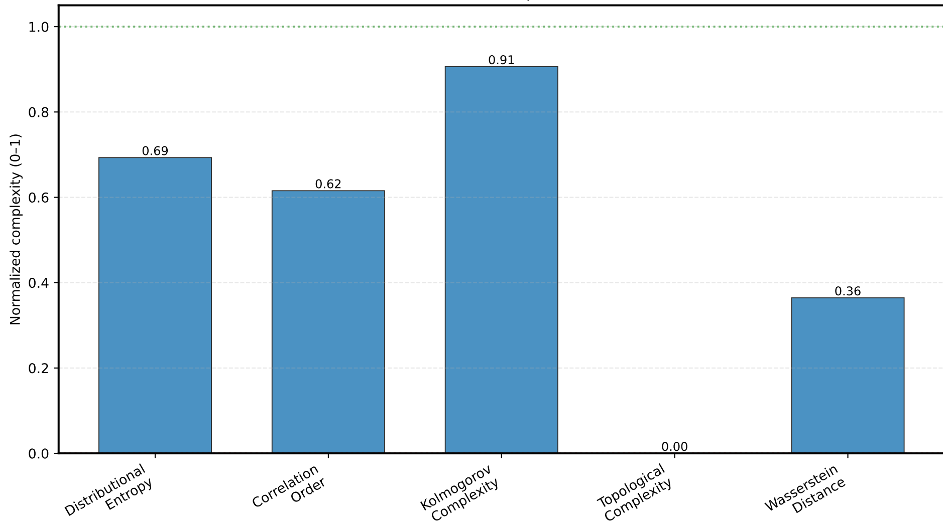
Normalized dataset complexities — moons
