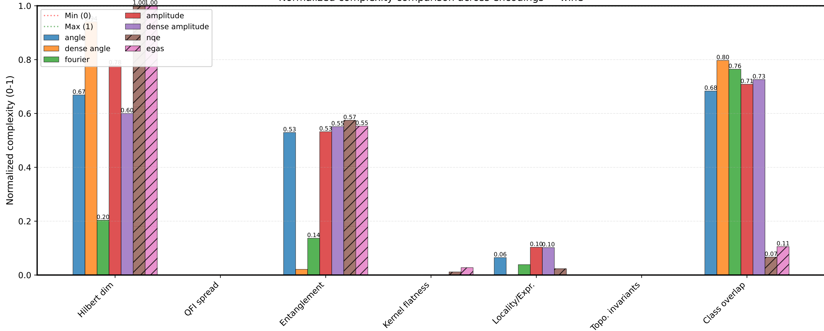
Normalized complexity comparison across encodings — wine
