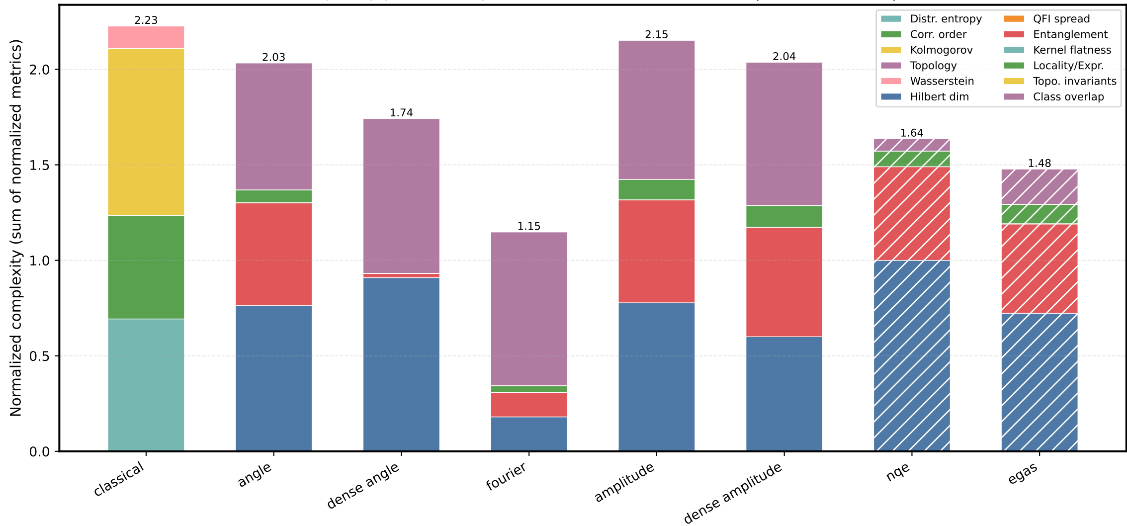
Dataset complexity per encoding (normalized metrics) — eurosat | classes: (0, 1) | PCA→8
