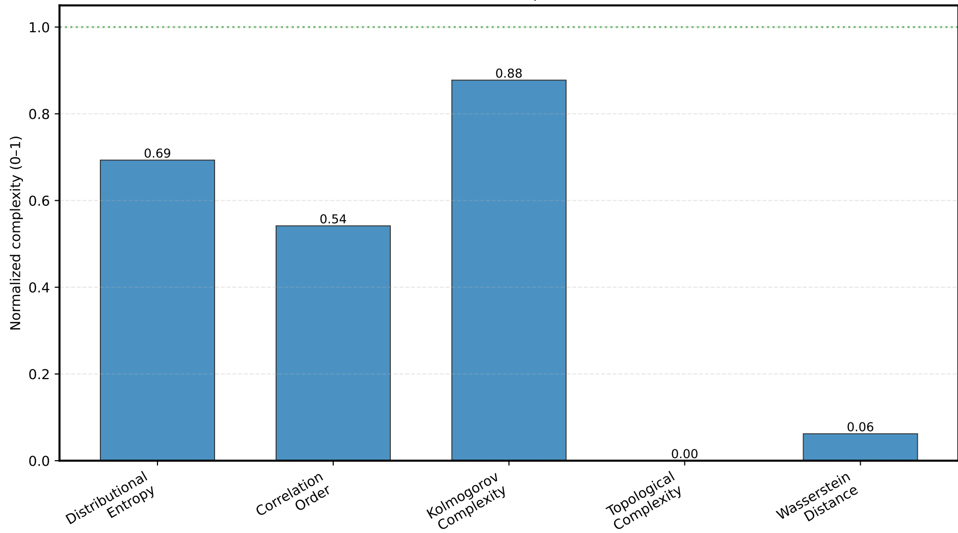
Normalized dataset complexities — cifar10
