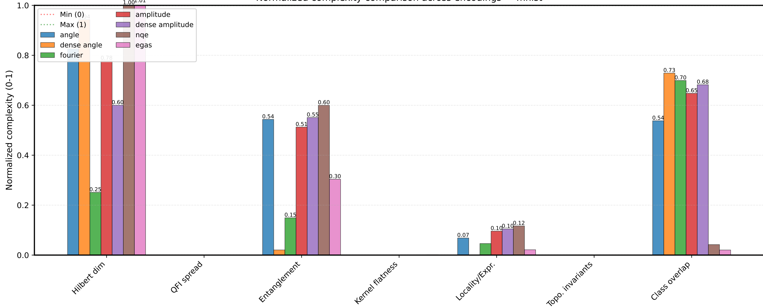
Normalized complexity comparison across encodings — mnist
