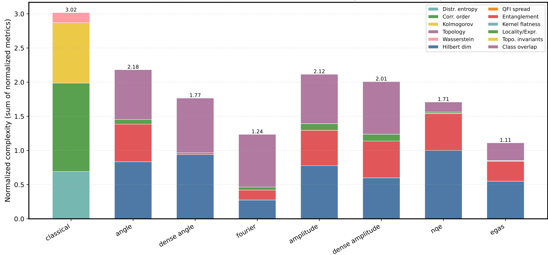
Dataset complexity per encoding (normalized metrics) — mnist | classes: (0, 1, 2, 3) | PCA→8
