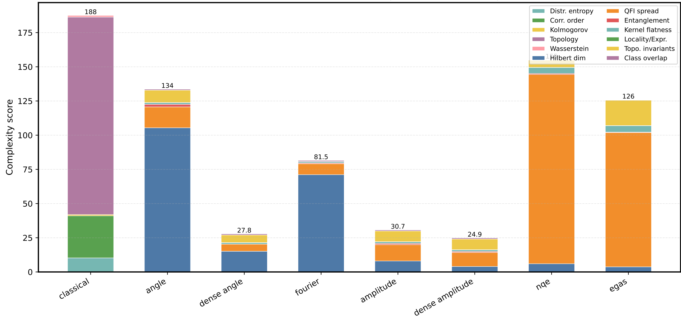
Dataset complexity per encoding — mnist | classes: (0, 1, 2, 3) | PCA→8
