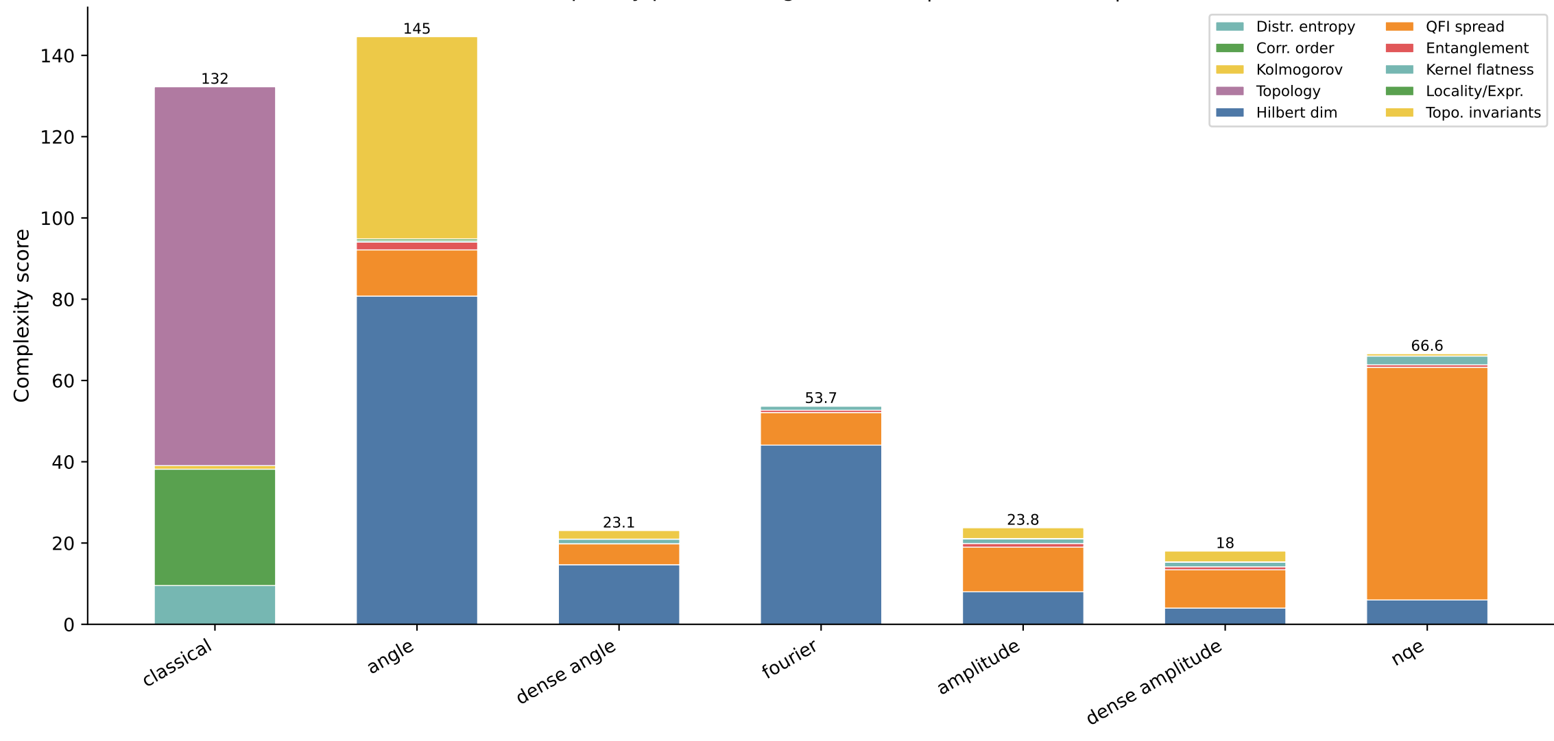
Dataset complexity per encoding — fashion | classes: (0, 1) | PCA→8
