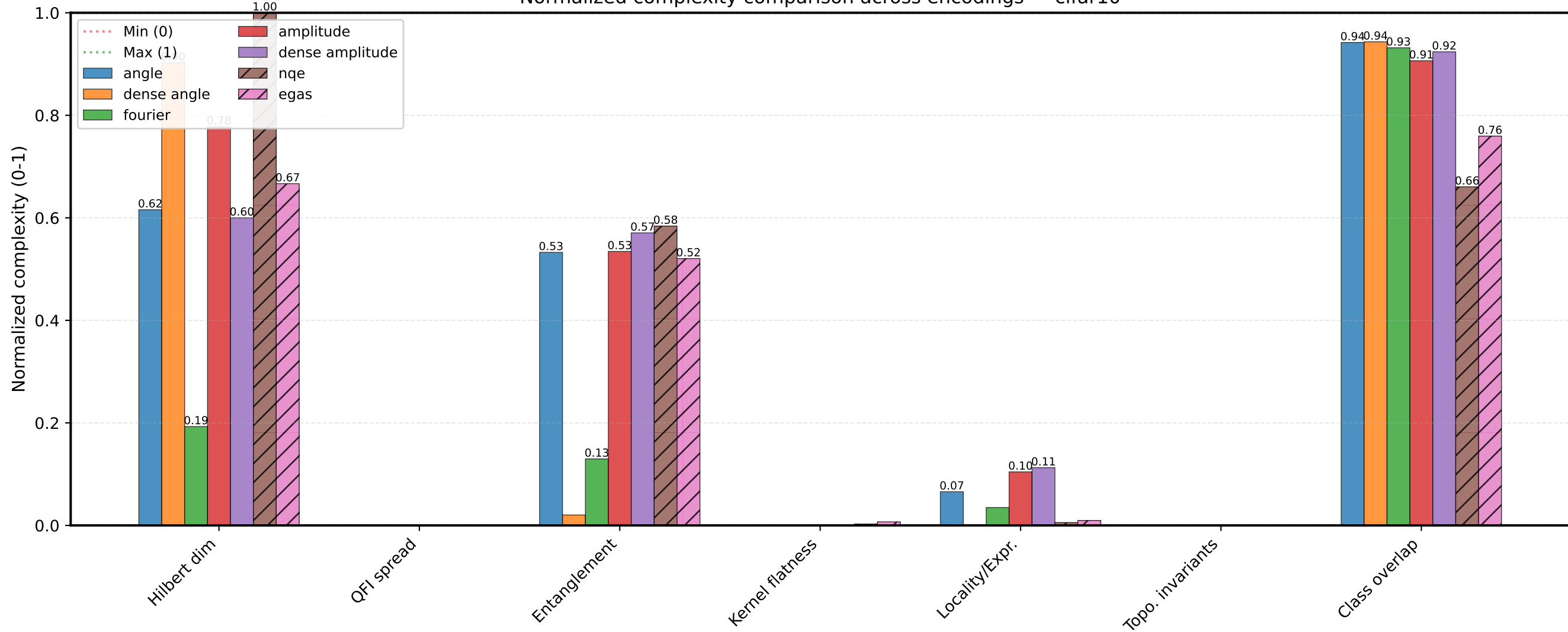
Normalized complexity comparison across encodings — cifar10
