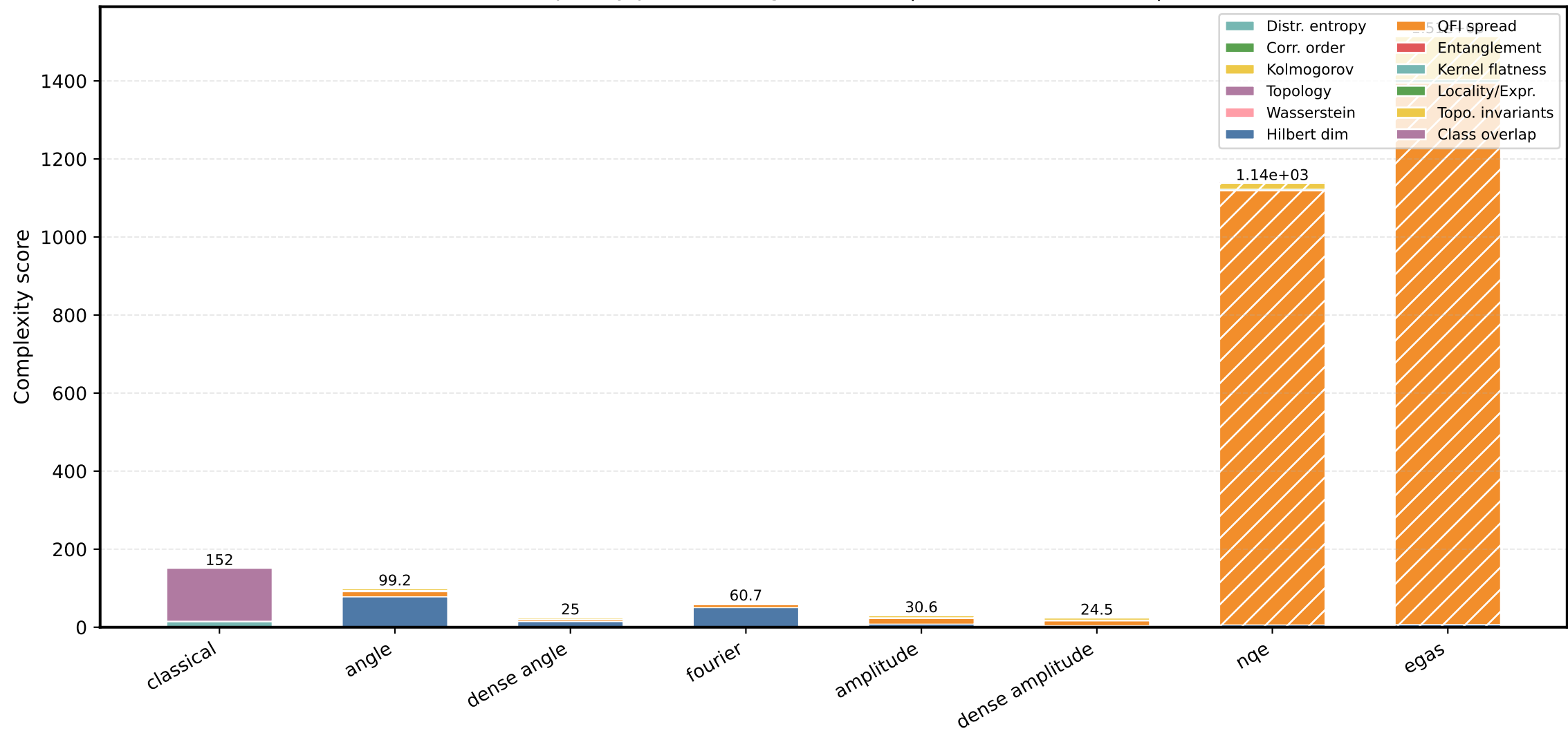
Dataset complexity per encoding — cifar10 | classes: (0, 1, 2, 3) | PCA→8
