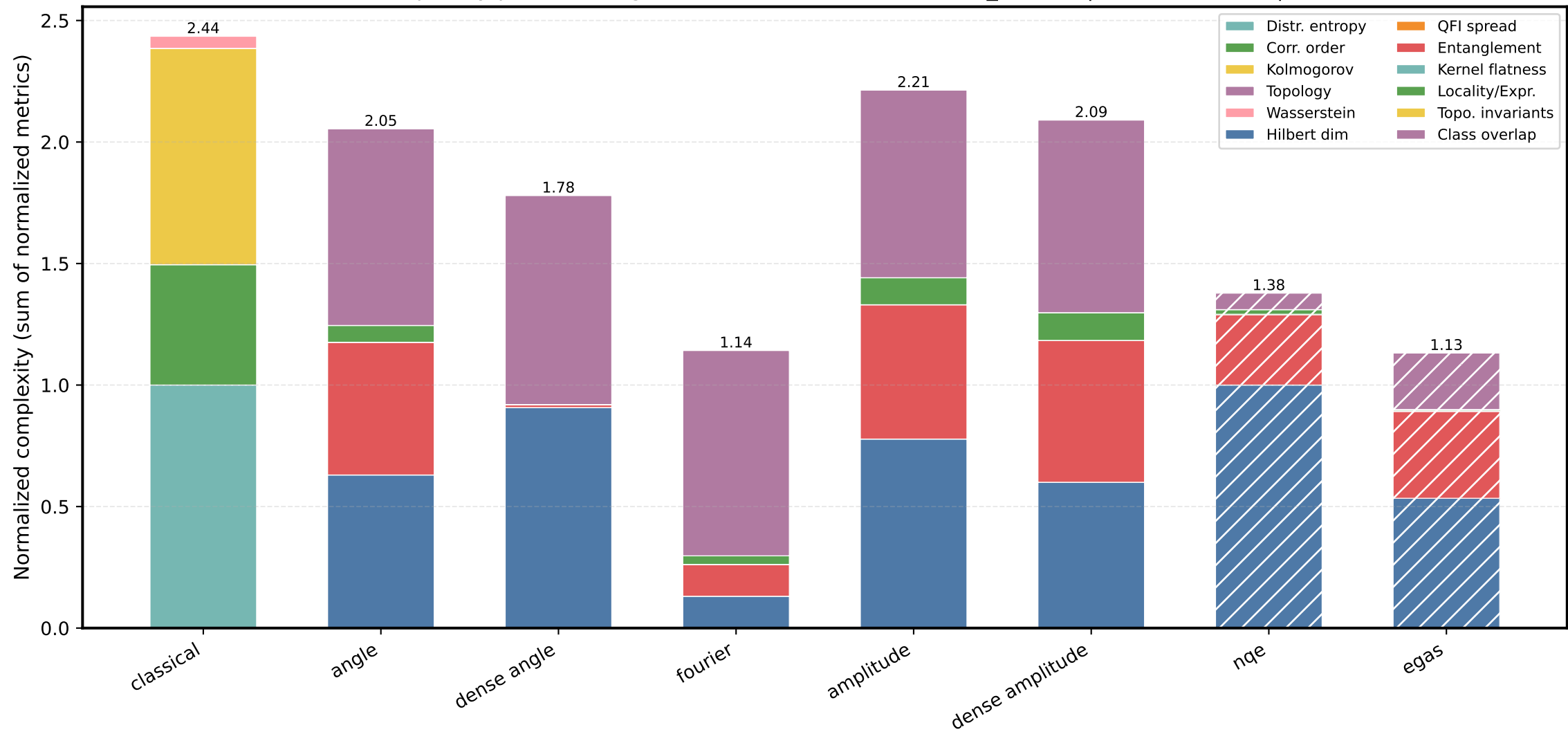
Dataset complexity per encoding (normalized metrics) — breast_cancer | classes: (0, 1) | PCA→8
