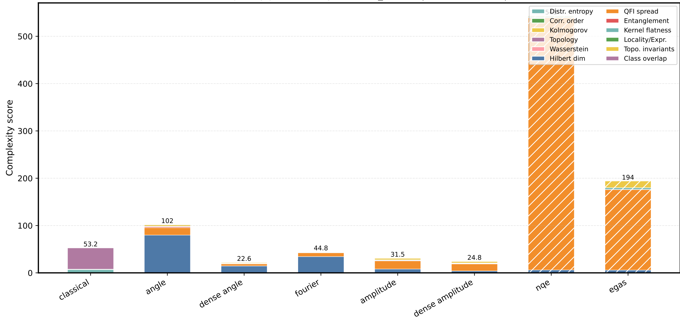
Dataset complexity per encoding — breast_cancer | classes: (0, 1) | PCA→8
