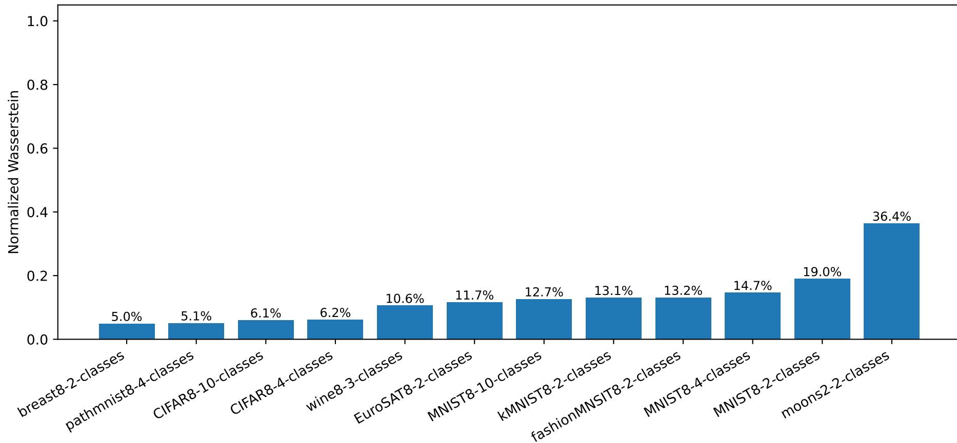
Normalized Classical Wasserstein Distance
