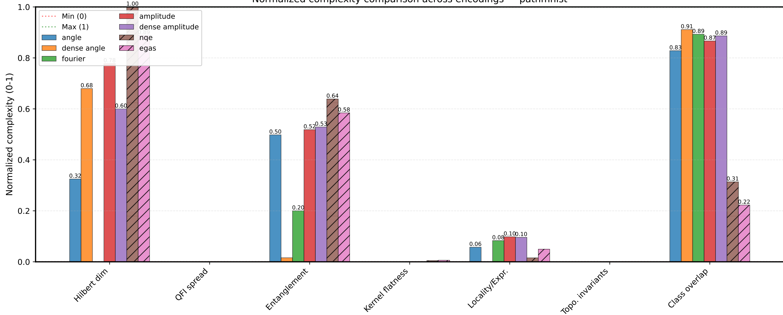
Normalized complexity comparison across encodings — pathmnist
