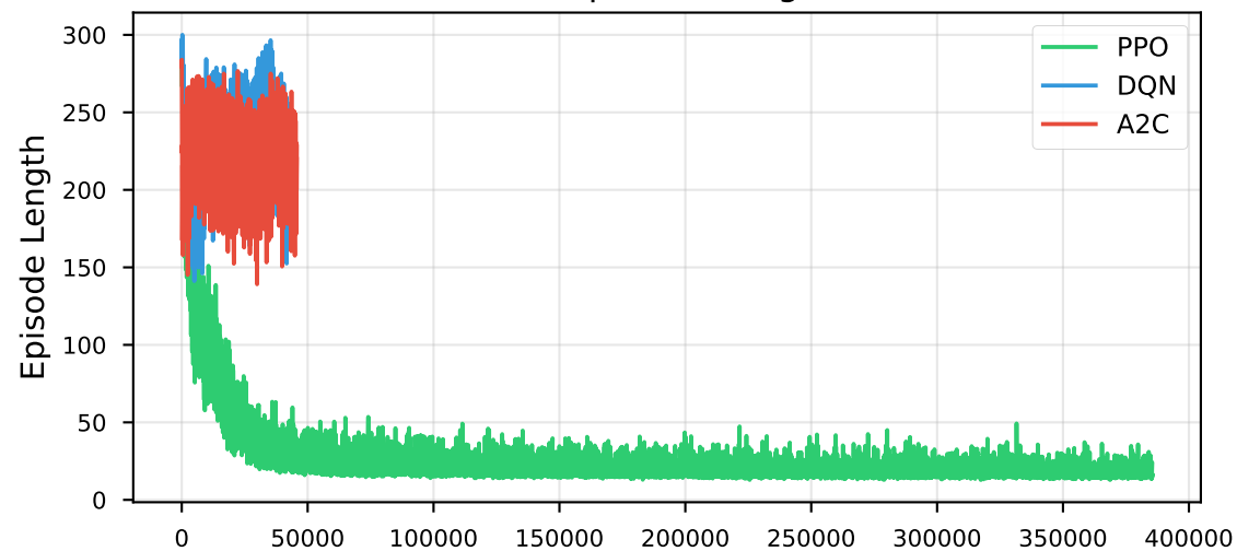
E3_FIXED: Episode Length
