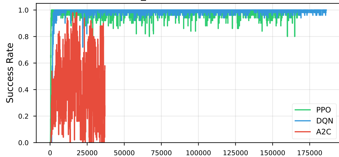
E4: Success Rate
