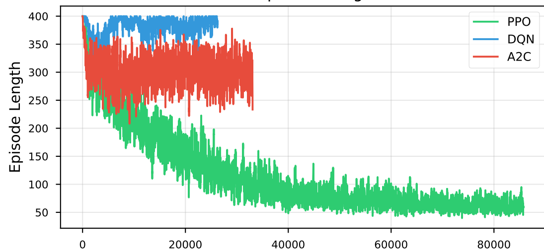
E5_FIXED: Episode Length
