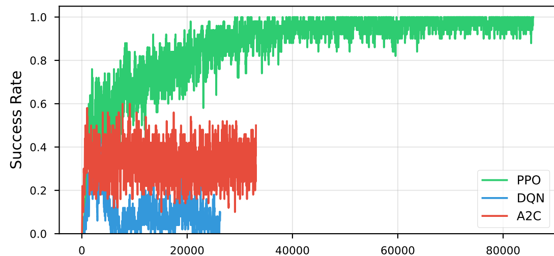
E5_FIXED: Success Rate
