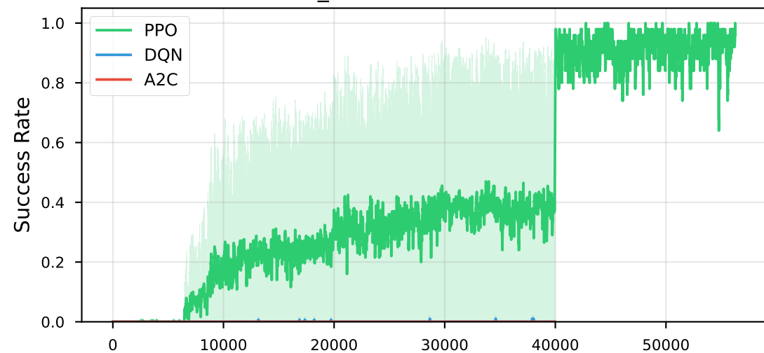
E6_RANDOM: Success Rate
