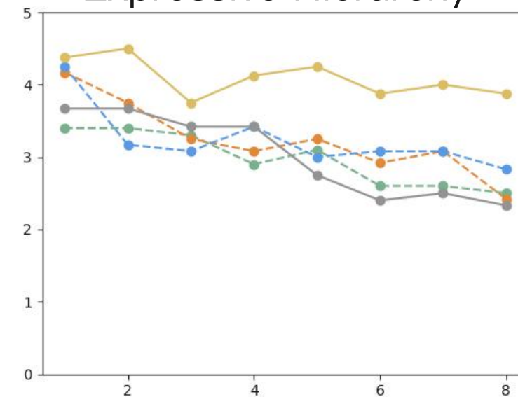
Expressive Hierarchy
