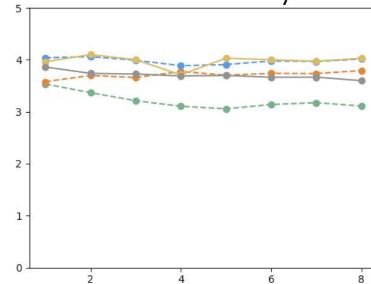
Sound Fidelity
