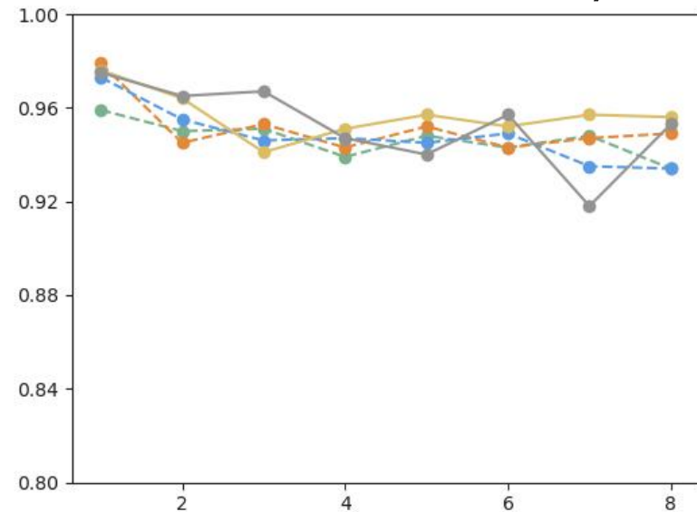
Timbre Consistency
