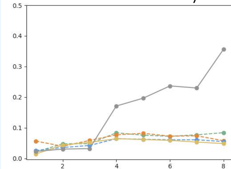
Content Accuracy
