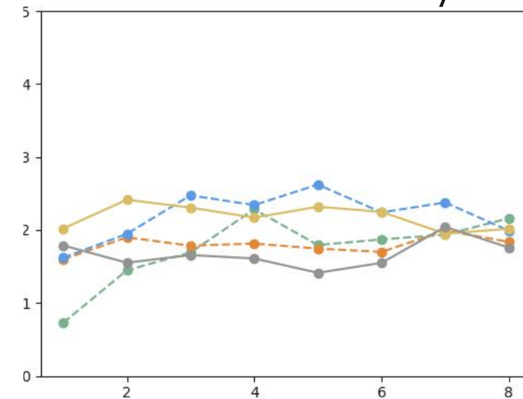
Reverb Consistency
