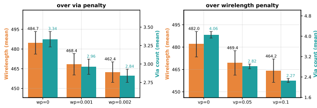
Figure 9: Reward weight sweep (3×3 factorial). Bars show marginal means with error bars. Wirelength: left axis (orange); via count: right axis (teal).
