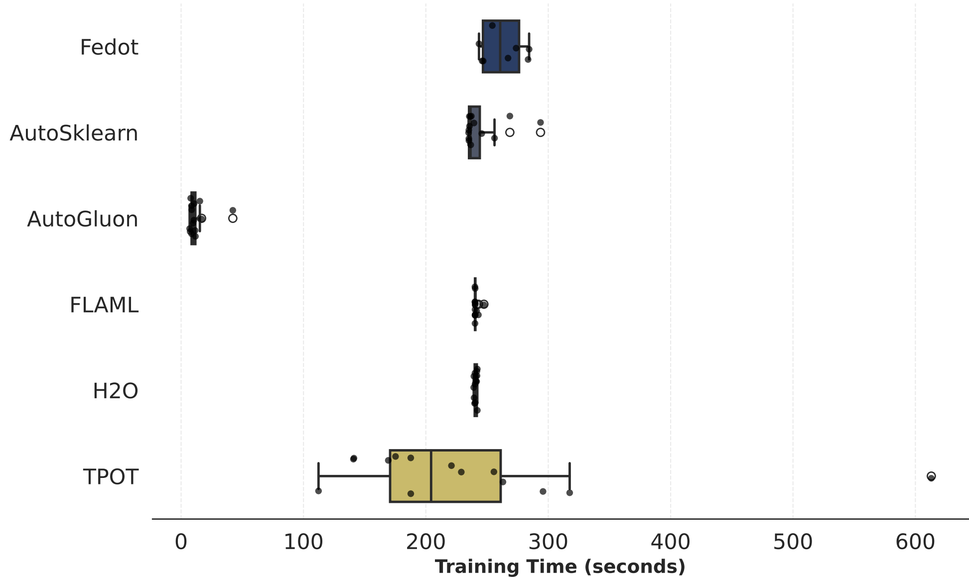
Training Time Distribution - f1_ (40 runs)
