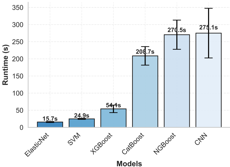
Average Runtime per Model
