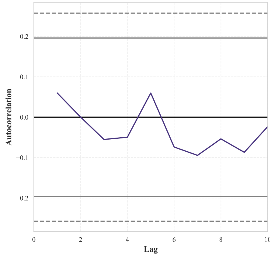
Residual Autocorrelation: Model_B
