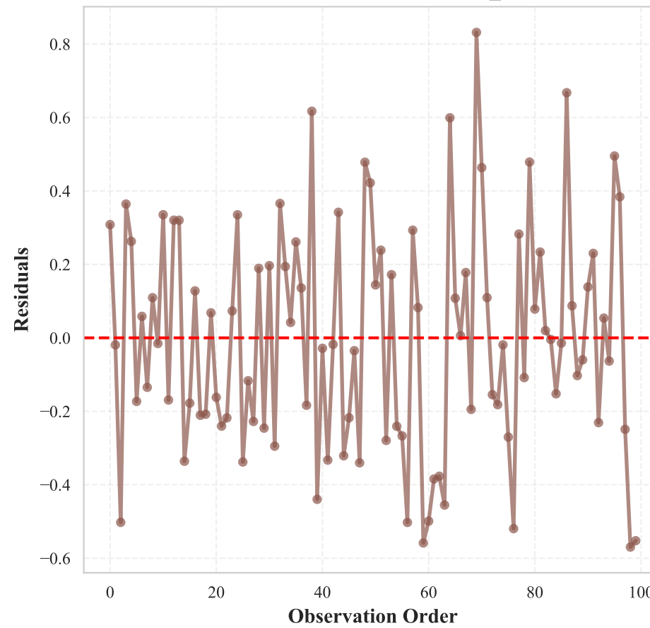
Residuals vs Order: Model_B
