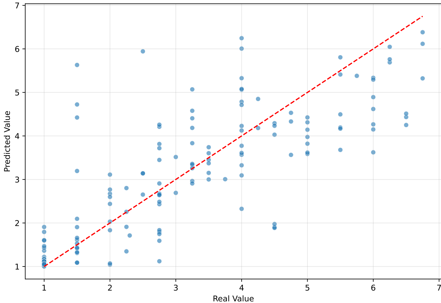
RandomForest MSE: 1.0388 - R 2 : 0.6601
